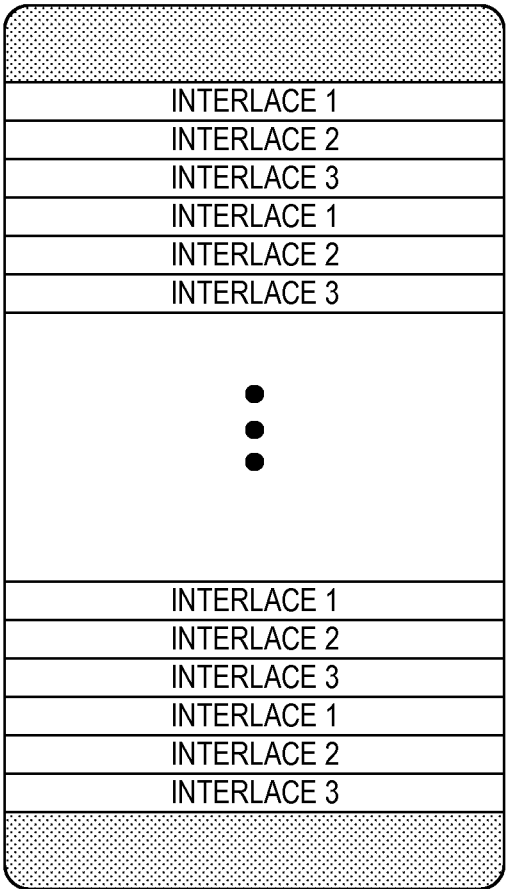
FIG. 1 An interlacing design for NR-U with 20MHz bandwidth, 60 KHz subcarrier spacing, and 3 interlaces
