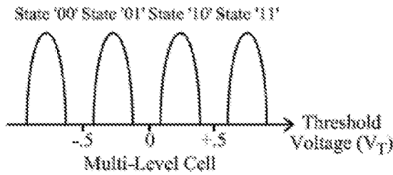
Multi-Level Cell FIG. 11B
