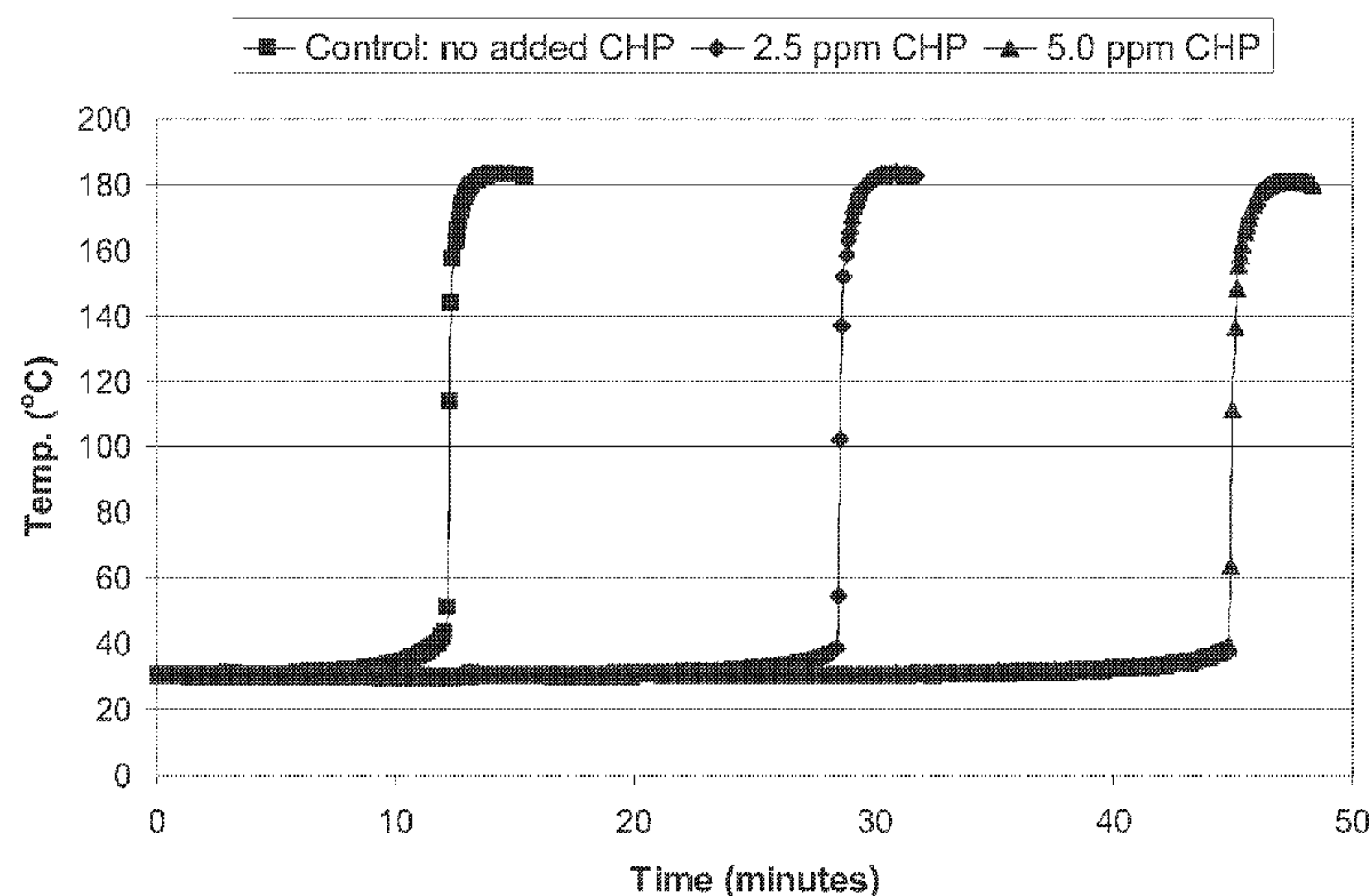
FIG. 1 Effect of Cumyl Hydroperoxide (CHP) on Exotherm Time
