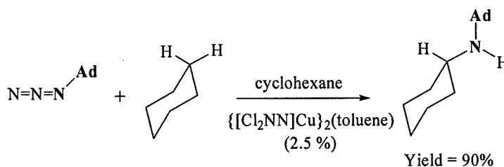
Scheme 13.
