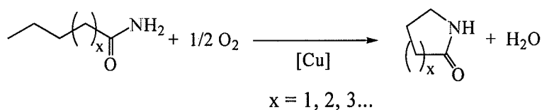
Scheme 35.
