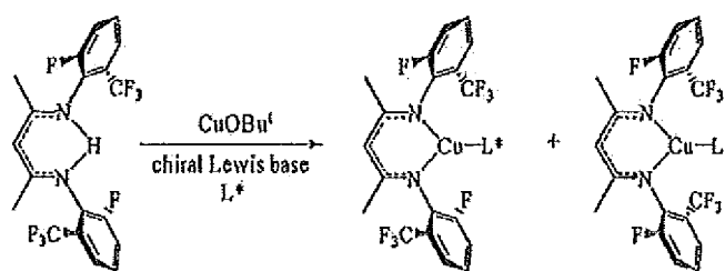
Scheme 38.
