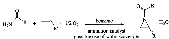
Scheme 34.
