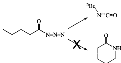
Scheme 37.
