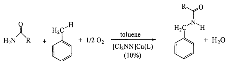
Scheme 33.
