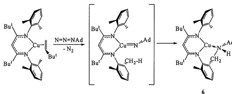
Scheme 9.
