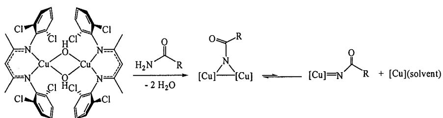
Scheme 32.
