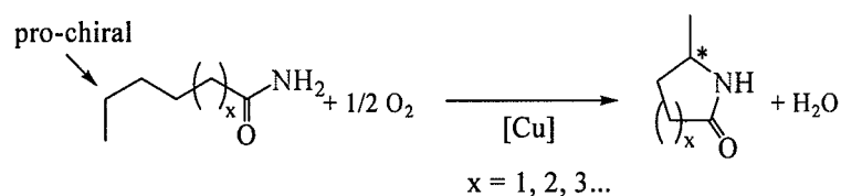
Scheme 36.
