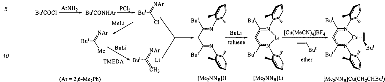
Scheme 8.
