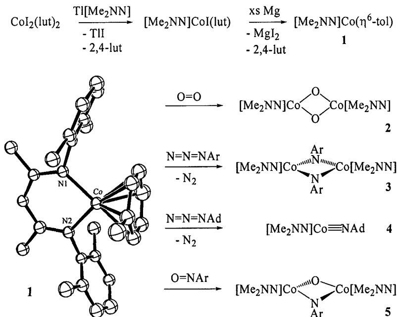
Scheme 7.
