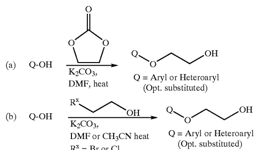
Scheme 1. Preparation of some starting materials
