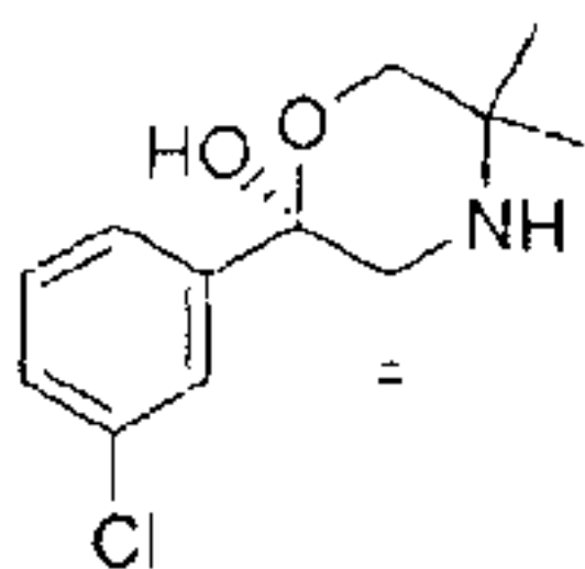
(R,R)-2-(3-Chlorophenyl)-2-hydroxy-3,5,5-trimethyl-morphinol
