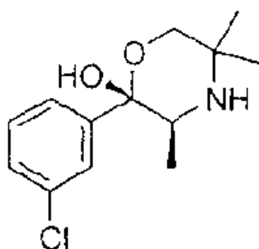
(S,S)-2-(3-Chlorophenyl)-2-hydroxy-3,5,5-trimethyl-morphinol
