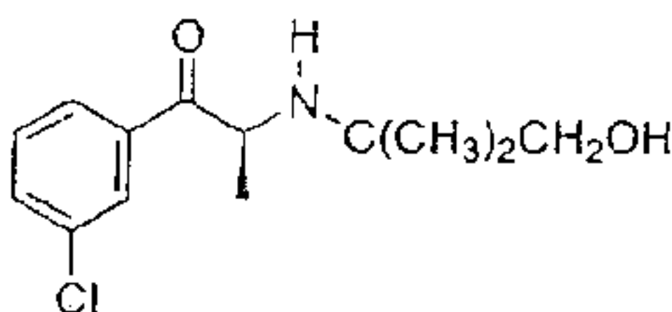
(S)-1-(3-Chlorophenyl)-2-[(1,1-dimethylethanol)amino]-1-propanone
