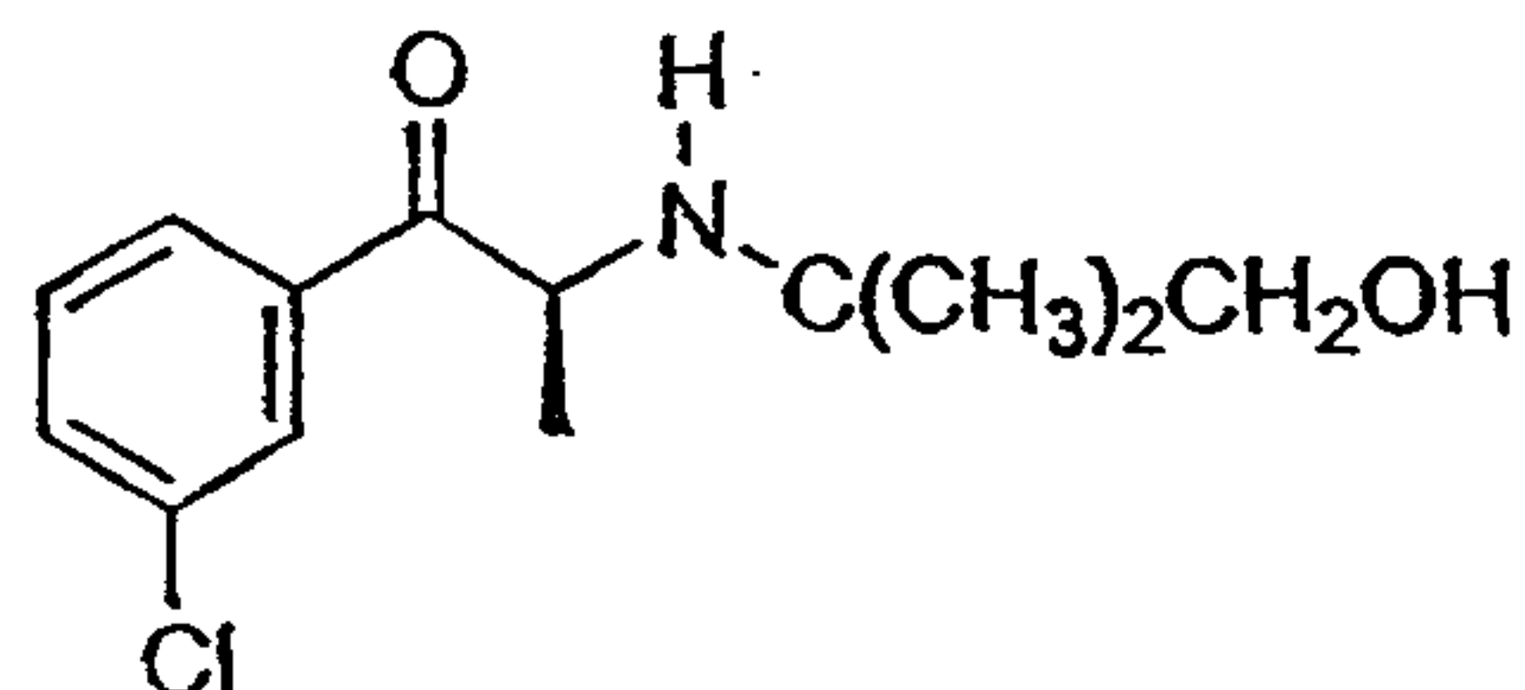
(S)-1-(3-Chlorophenyl)-2-[(1,1-dimethylethanol)amino]-1-propanone
