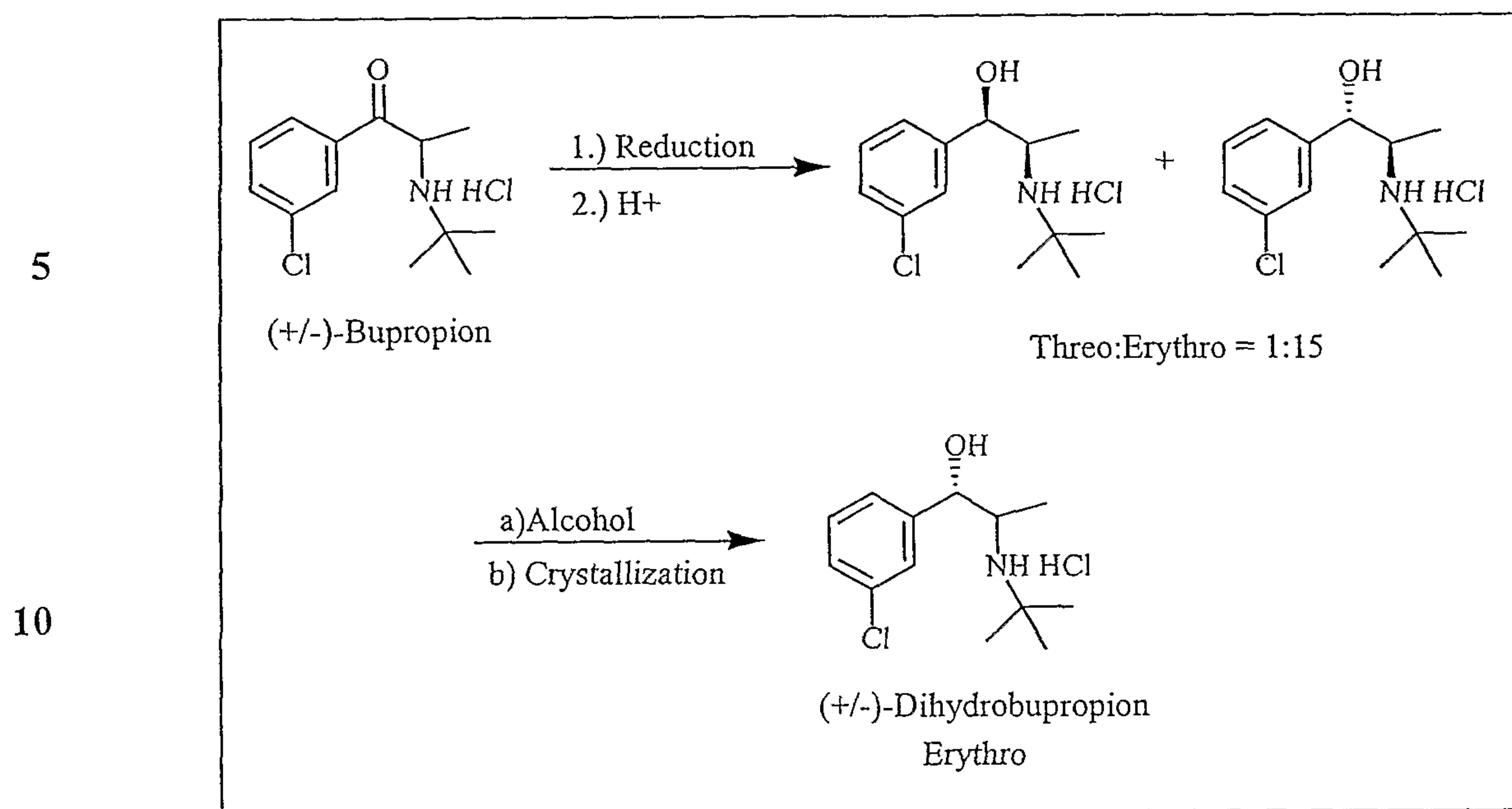
Scheme 6
