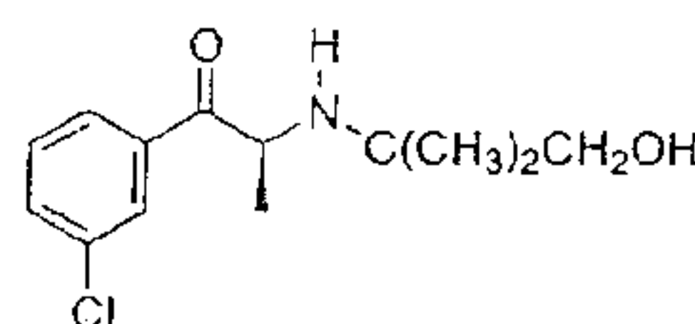
(S)-1-(3-Chlorophenyl)-2-[(1,1-dimethylethanol)amino]-1-propanone
