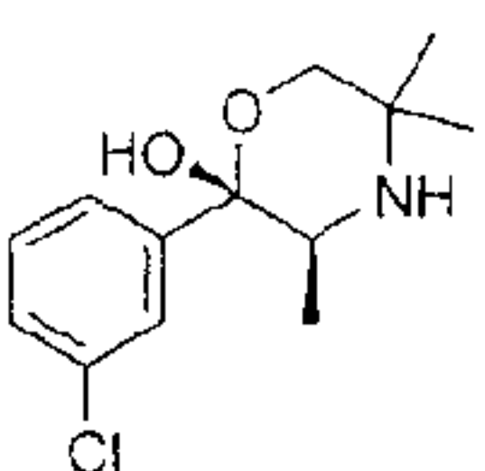
(S,S)-2-(3-Chlorophenyl)-2-hydroxy-3,5,5-trimethyl-morphinol
