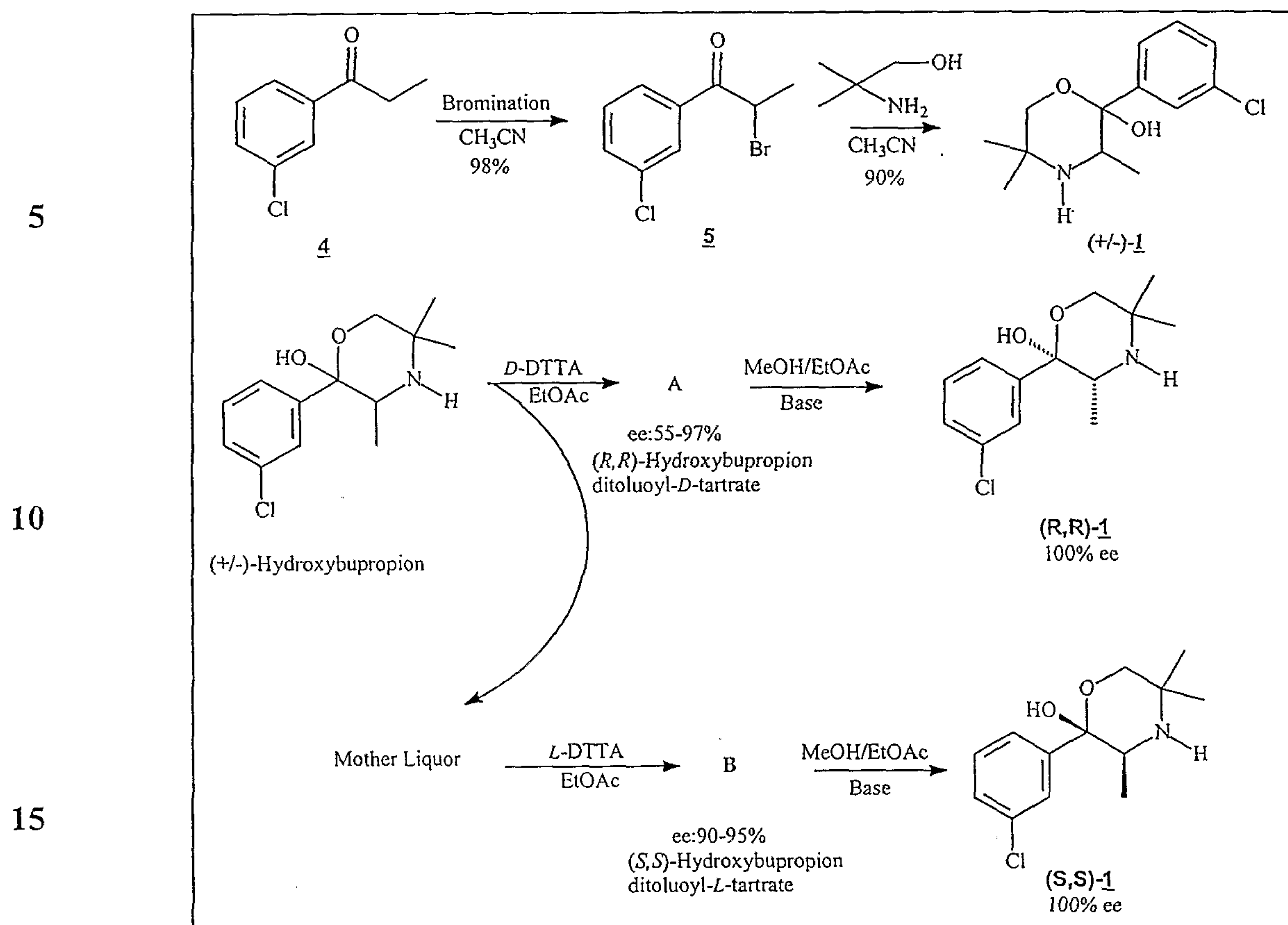
Scheme 4
