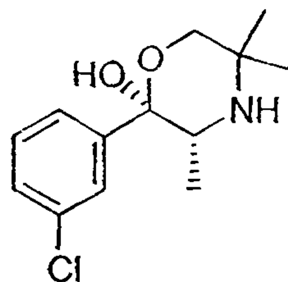
(R,R)-2-(3-Chlorophenyl)-2-hydroxy-3,5,5-trimethyl-morpholinol
