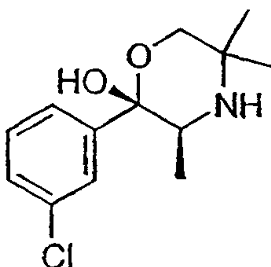
(S,S)-2-(3-Chlorophenyl)-2-hydroxy-3,5,5-trimethyl-morpholinol
