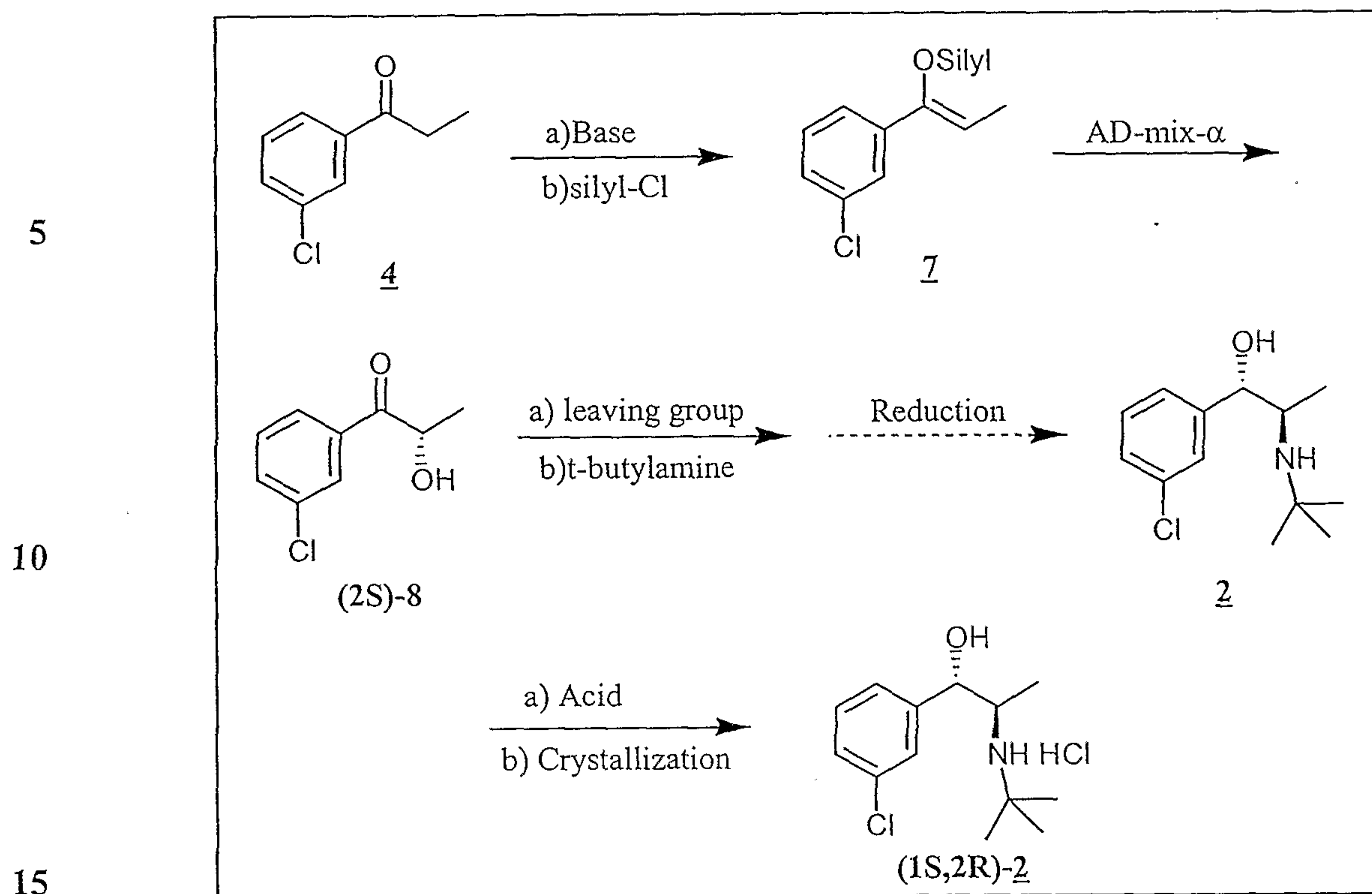
Scheme 7
