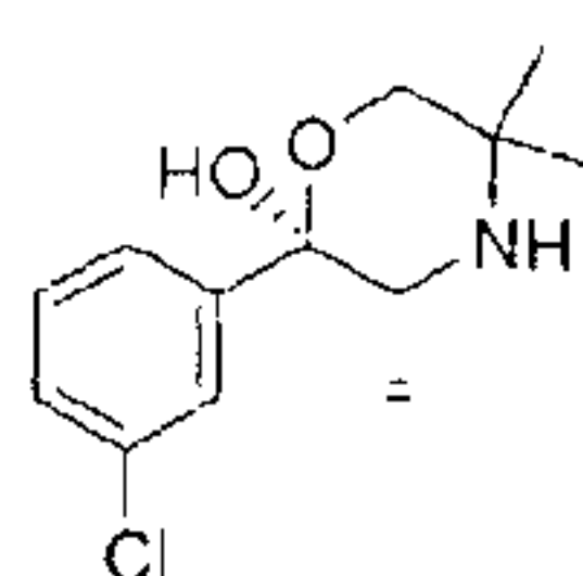
(R,R)-2-(3-Chlorophenyl)-2-hydroxy-3,5,5-trimethyl-morphinol
