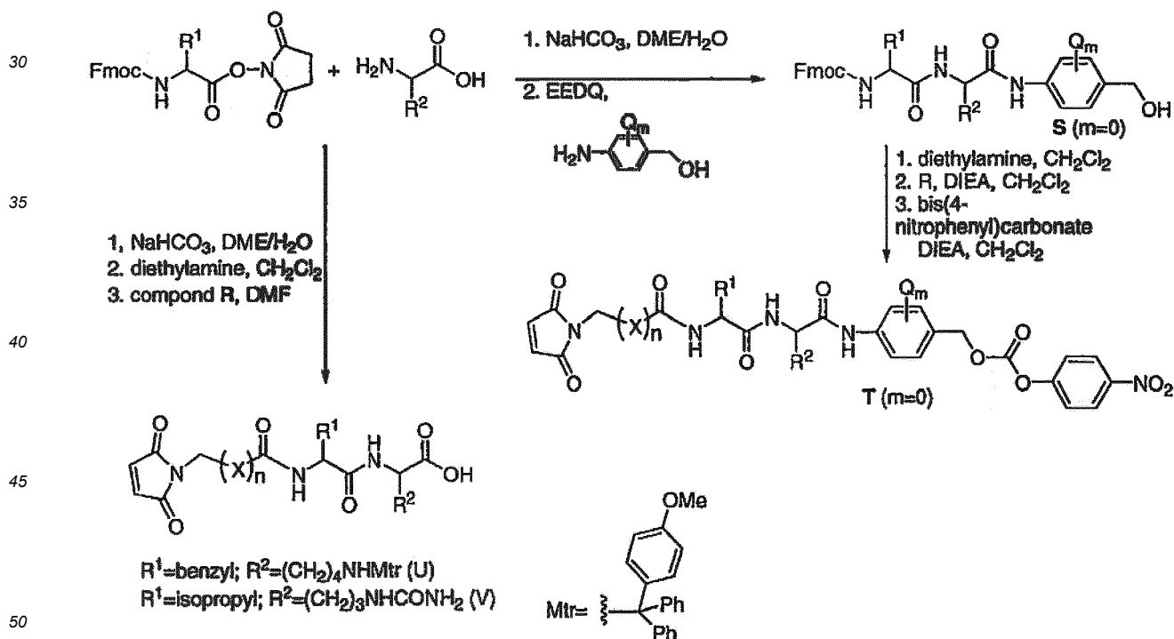
Scheme 10
