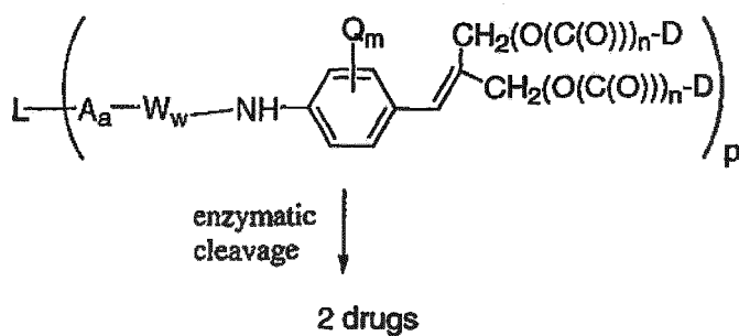
Scheme 4
