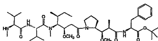
MeVal-Val-Dil-Dap-Phe-OtBu, 1001
