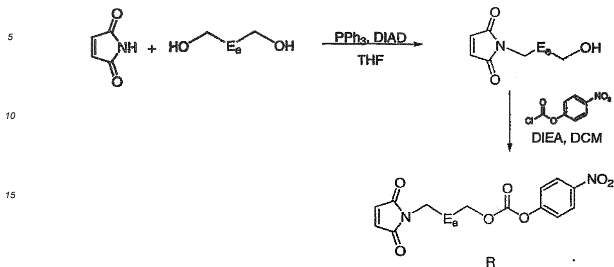
Scheme 9
