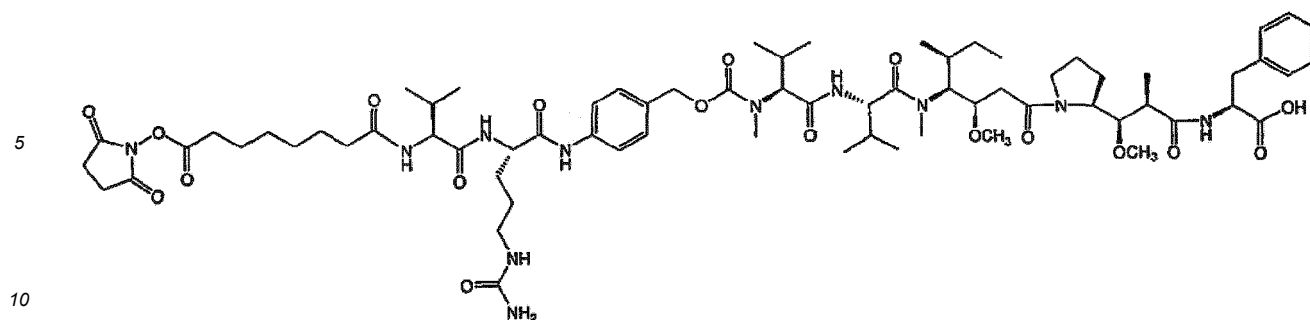
Compound 17
