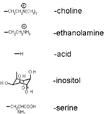
Scheme 1: Functional groups in phospholipids
