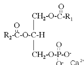
Calcium Salt of Phosphatidic Acid
