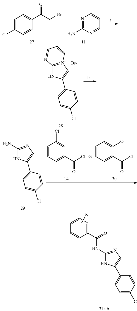
Scheme 5. Synthesis of Series II compounds 31a-
