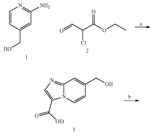
Scheme 1. Synthesis of Series I compounds 9a-d.
