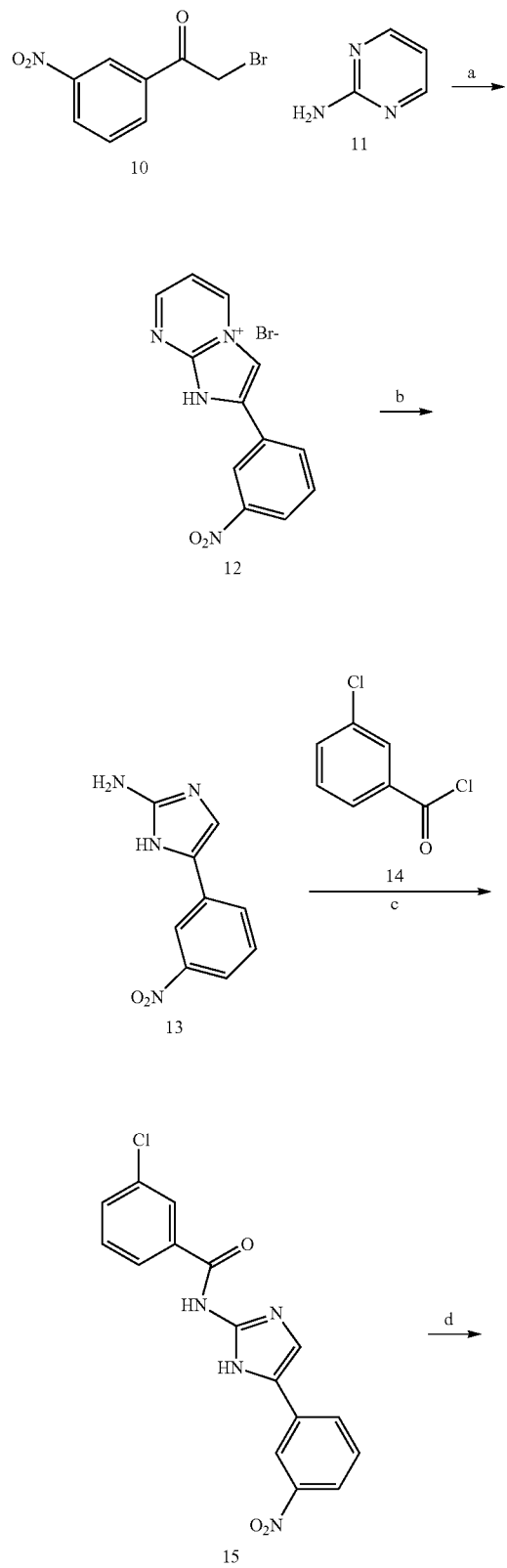
Scheme 2. Synthesis of Series II compounds 15 and 16.
