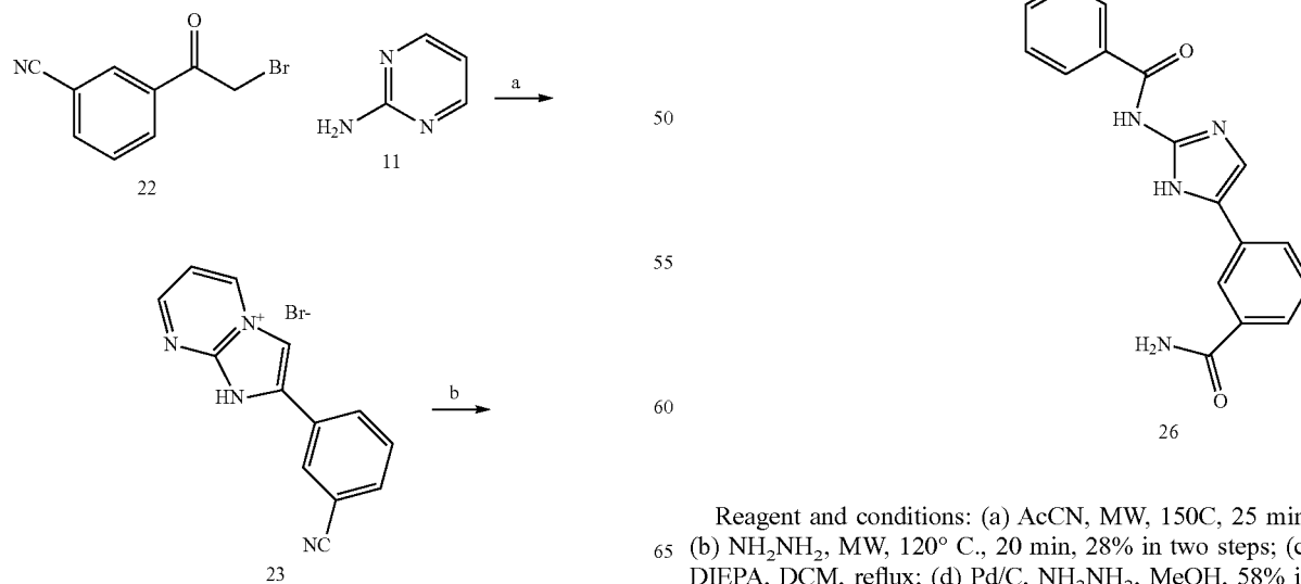
Scheme 4. Synthesis of Series II compounds 25 and 26.
