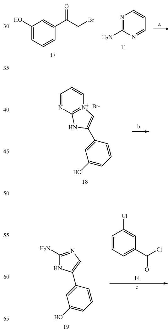
Scheme 3. Synthesis of Series II compounds 21.
