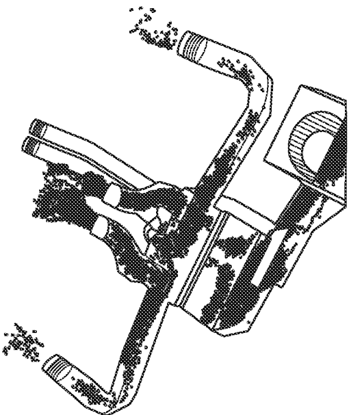
Noise Sources Distribution at 200Hz
