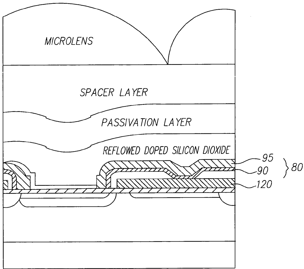
FIG. 3 (Prior Art)
