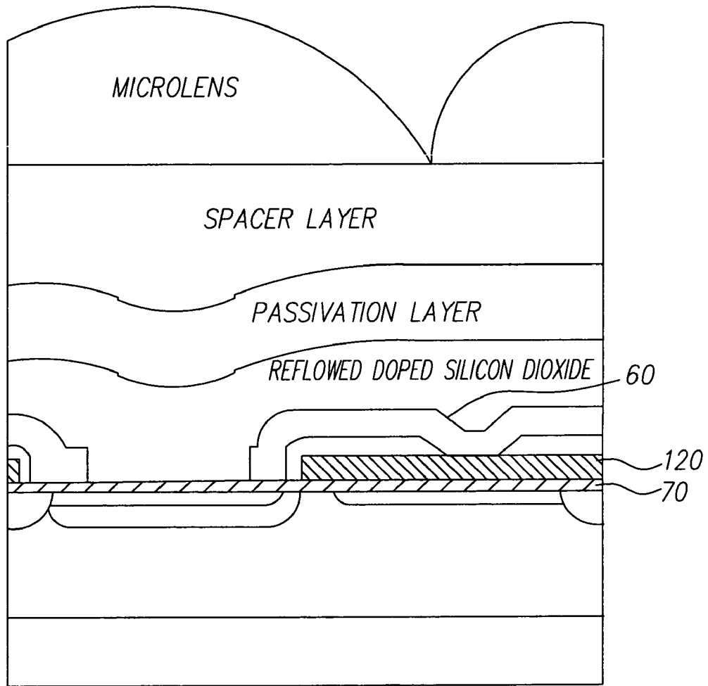
FIG. 2 (Prior Art)
