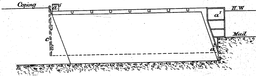
Long d Section of Dam showing Wall built up to High Water (by Mode N o 2)
