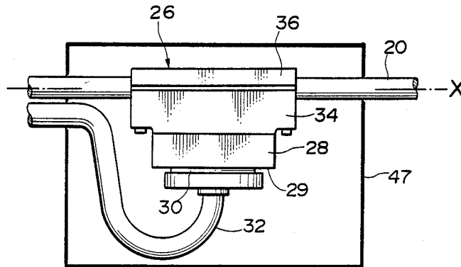
FIG. 5 (PRIOR ART)
