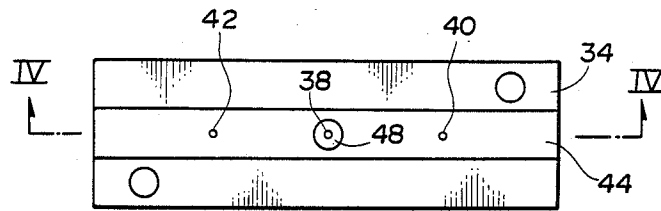
FIG. 3 (PRIOR ART)
