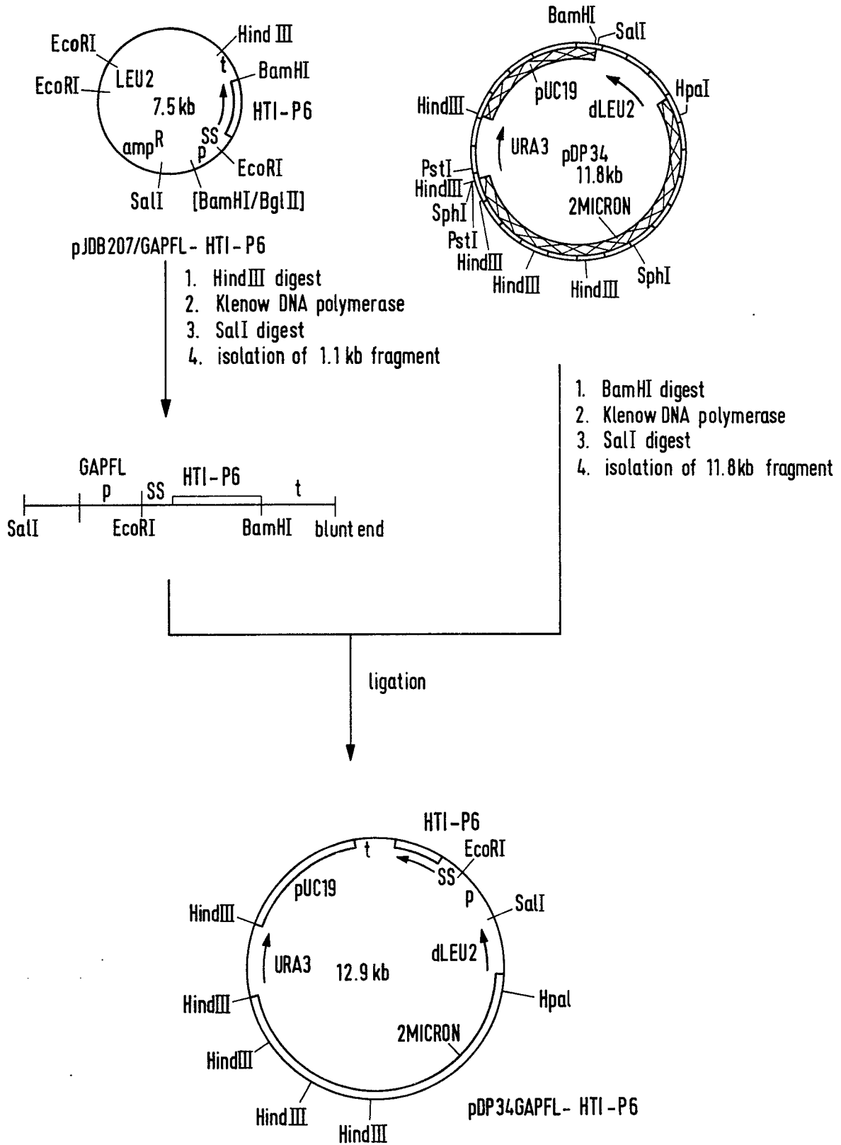
Fig. 5: Construction of plasmid pDP34/GAPFL - HTI - P6
