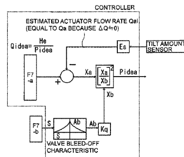
F7-a: HORSE POWER CALCULATION FUNCTION F7-b: OPERATION AMOUNT
