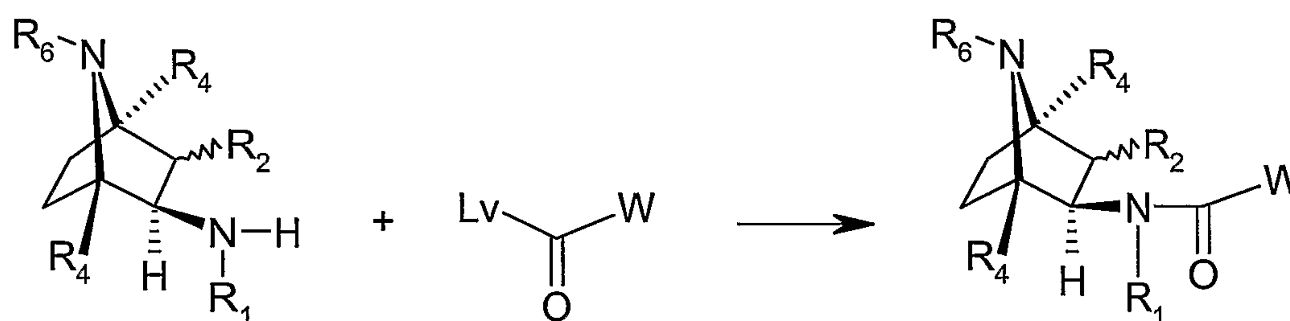
Scheme 1
