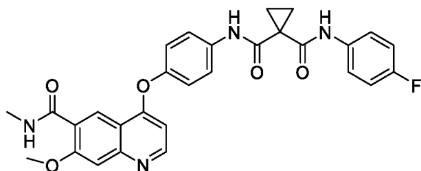
Compound 1
