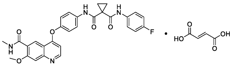
Compound 1 Fumarate
