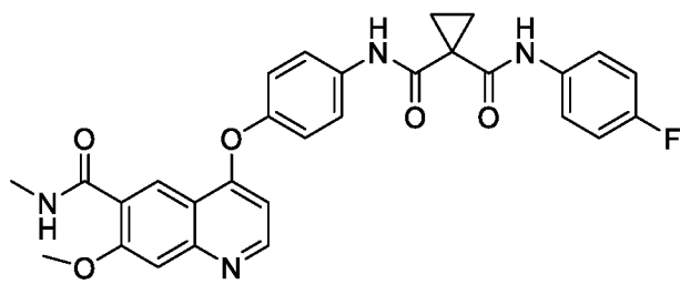
Compound 1
