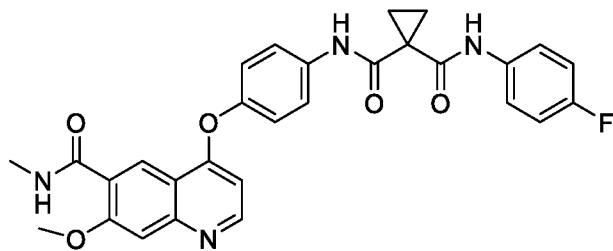
Compound 1
