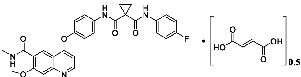
Compound 1 Hemifumarate
