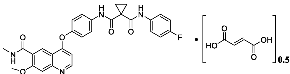
Compound 1 Hemifumarate
