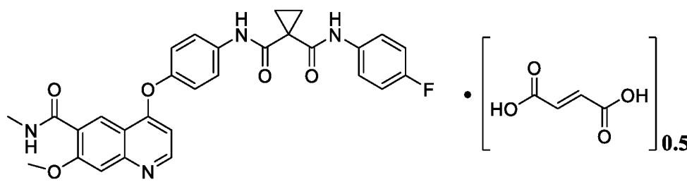
Compound 1 Hemifumarate
