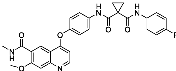
Compound 1
