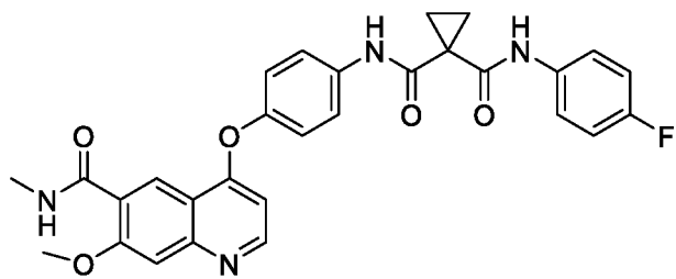
Compound 1
