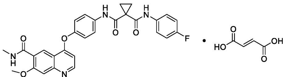
Compound 1 Fumarate
