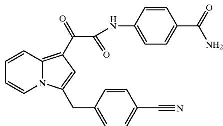
Compound (15)
