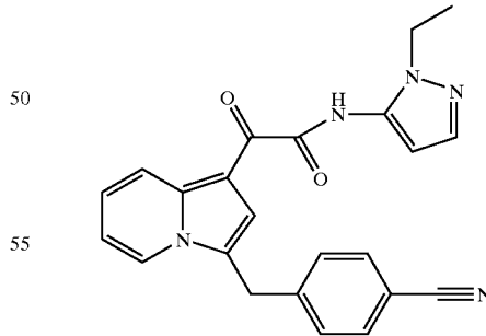
Compound (11)
