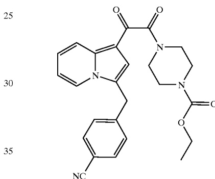
Compound (17)
