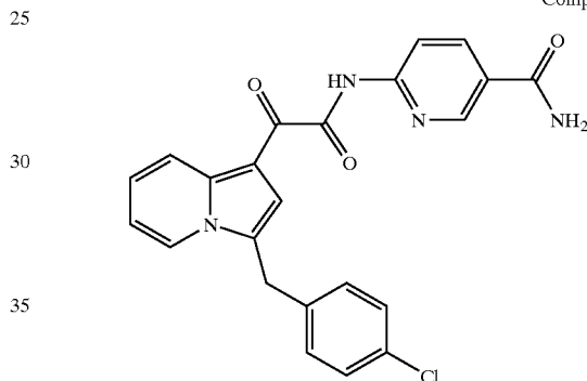
Compound (13)
