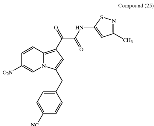
2-[3-(4-Cyano-benzyl)-6-nitro-indolizin-1-yl]-N-(3-methyl-isothiazol-5-yl)-2-oxo-acetamide
