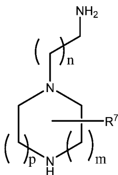
Structure II
