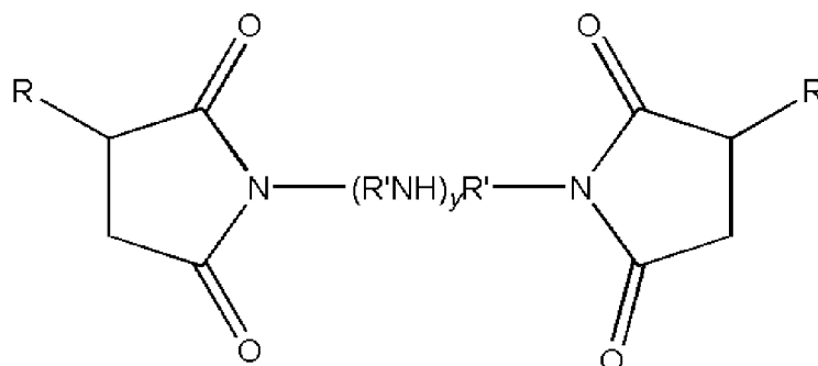
Structure VI
