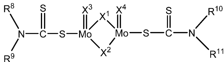
Structure IV
