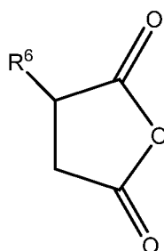
Structure I
