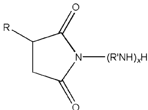
Structure VI
