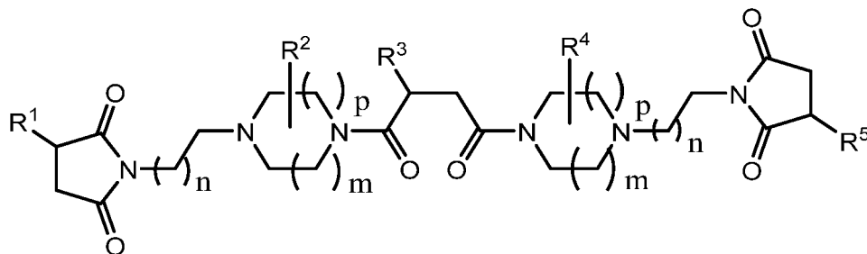
Structure III
