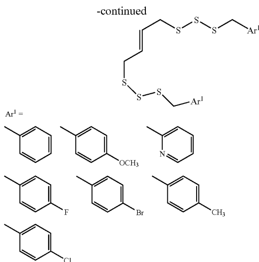
Scheme 6. Synthesis of tri-, tetra- and pentasulfide derivatives
