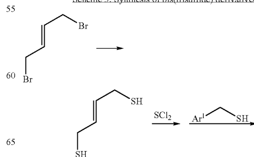
Scheme 5. Synthesis of bis(trisulfide) derivatives
