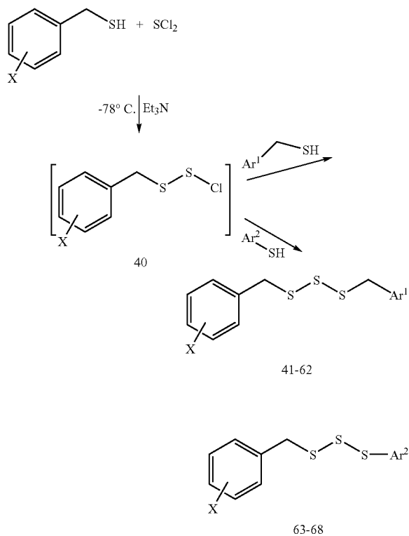
Scheme 3. Synthetic the symmetric trisulfides by Method B
