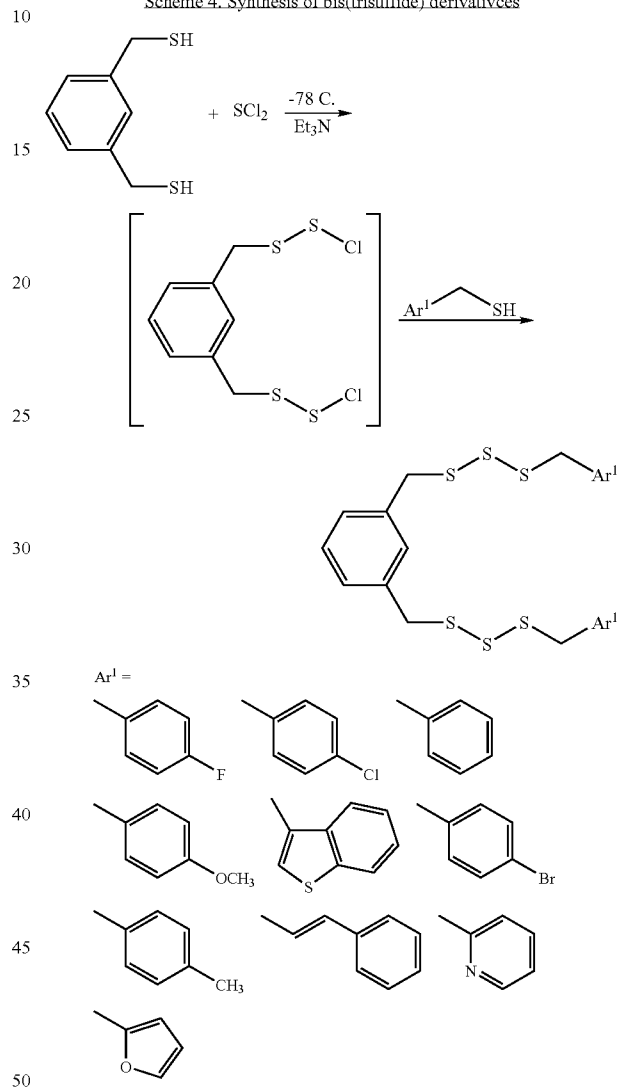
Scheme 4. Synthesis of bis(trisulfide) derivatives
