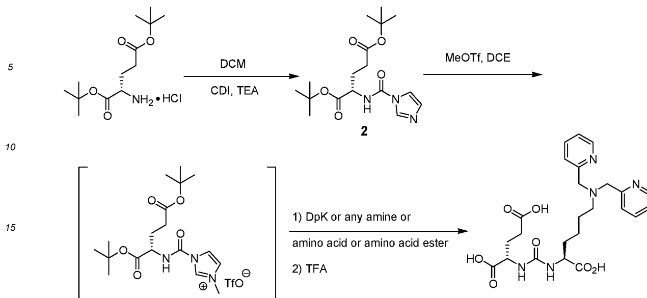
Scheme 1. General pathway for the synthesis of PSMA compounds.
