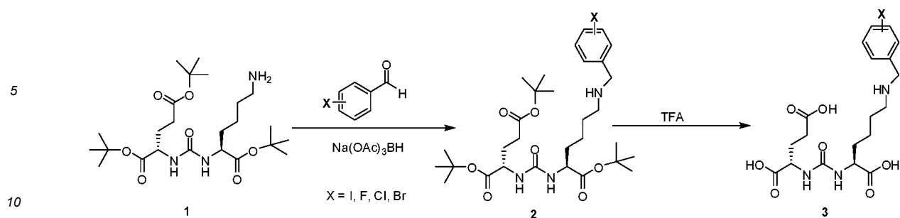
15 Scheme A. General pathway for the synthesis of halogenated Glu-Urea-Lys( N -benzyl-X) analogs (3).
