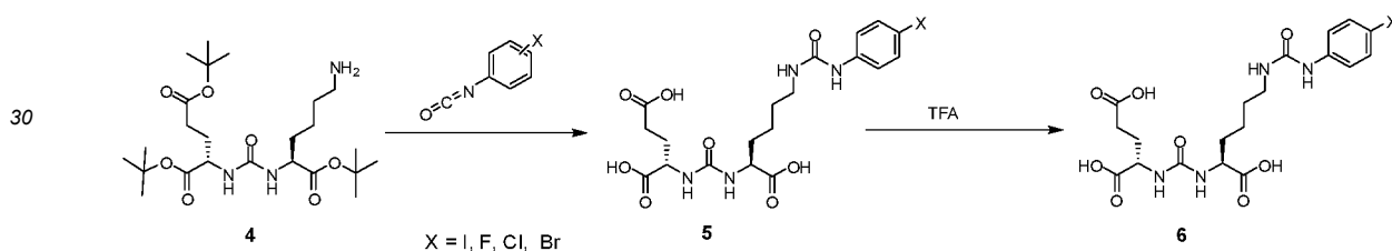
35 Scheme B. General pathway for the synthesis of halogenated Glu-Urea-Ureido(Phenyl-X) analogs.
