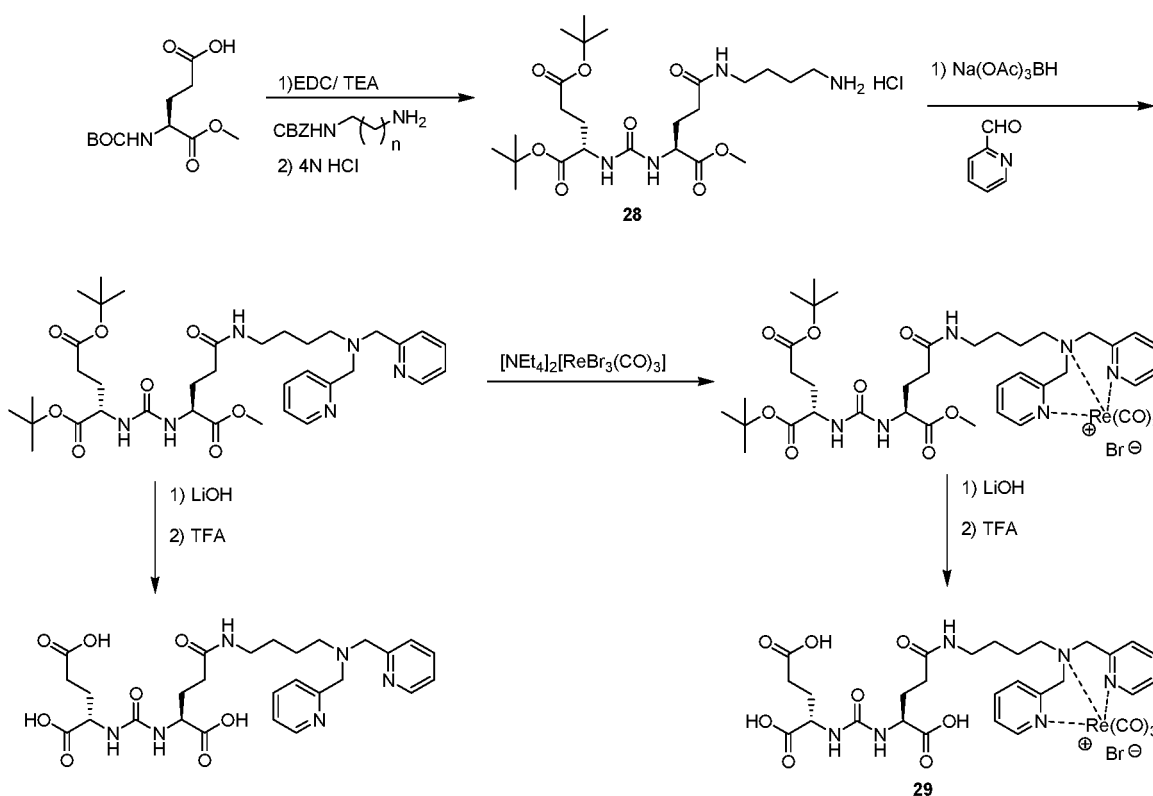
Scheme 4.
