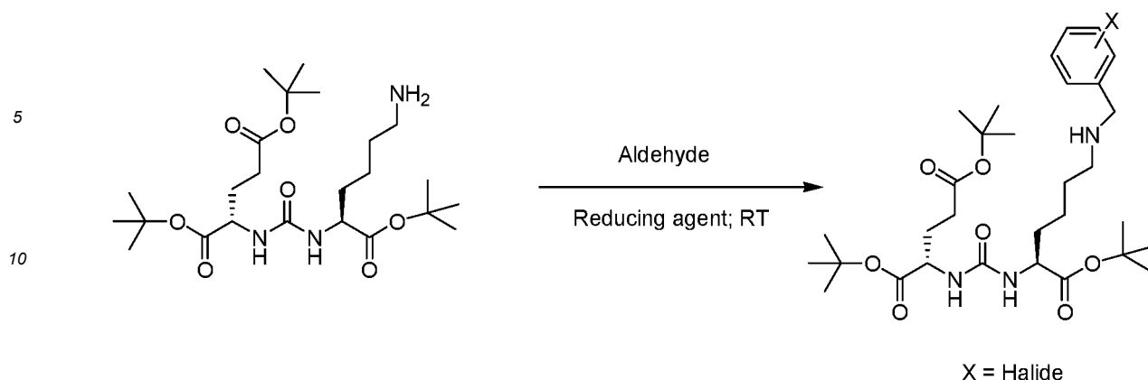
15 Scheme 3. General pathway for the synthesis of halogenated PSMA compounds.
