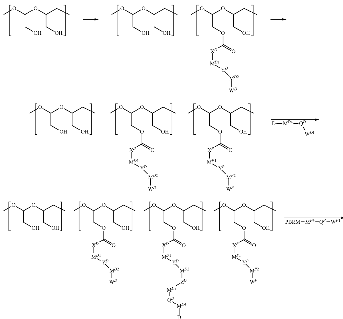
Scheme 5A
