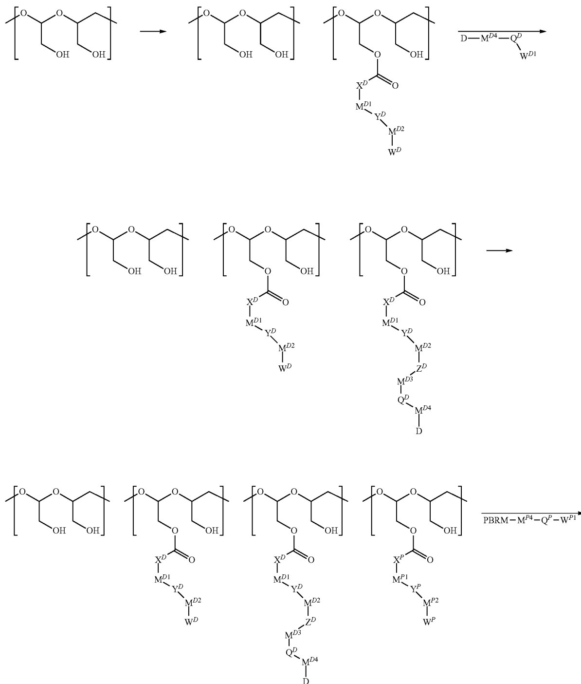
Scheme 5
