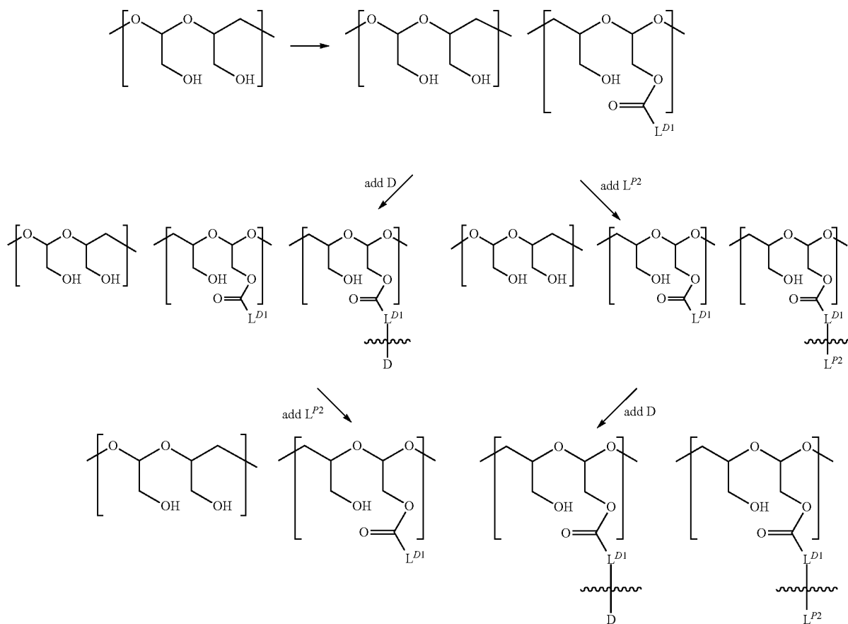
Scheme 10
