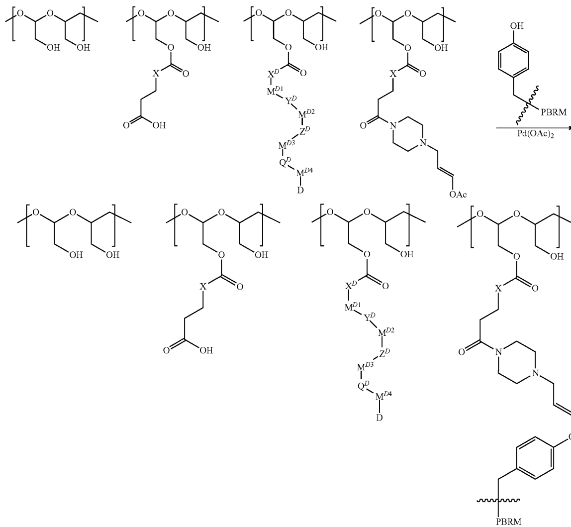
Scheme 9
