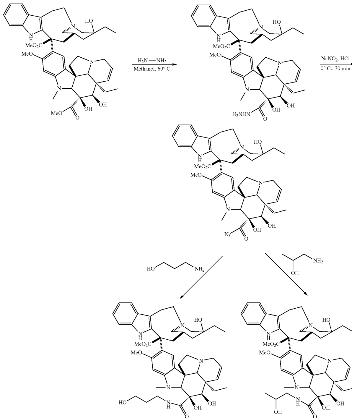
Scheme 1
