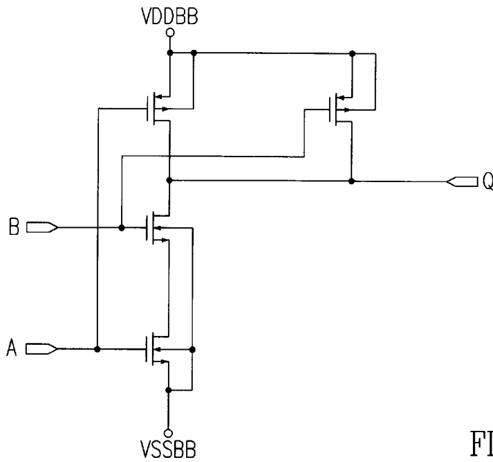
NAND2
