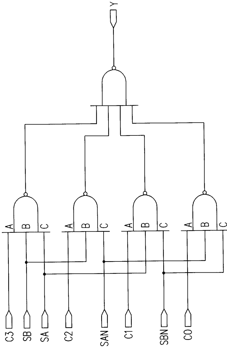
4:1 SELECTOR
