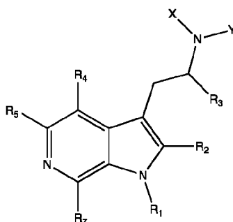
Formula If
