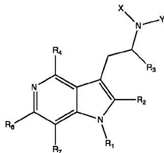
Formula Ia
