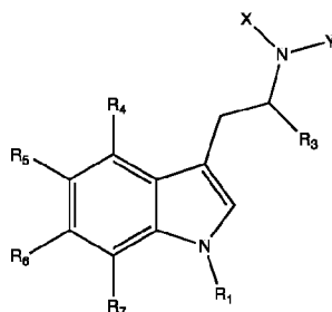
Formula Ih
