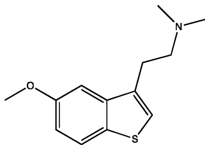
Bufothiophene™
