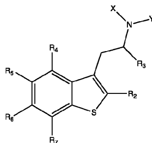
Formula Ia
