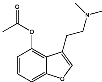
Furanopsilacetin™
