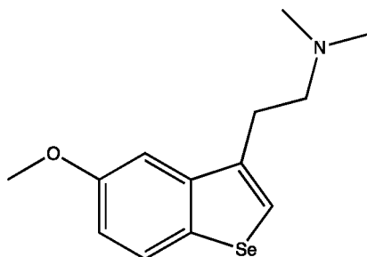
Bufoselenophene™
