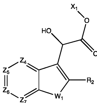
Formula IV
