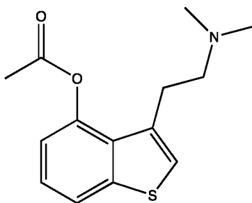
Thiopsilacetin™
