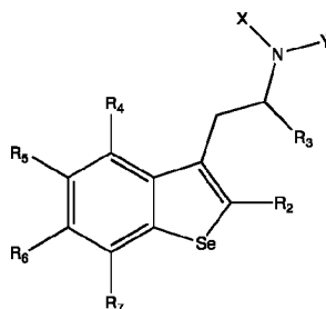
Formula Ib
