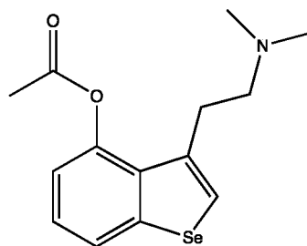
Selenopsilacetin™
