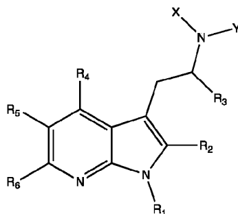
Formula Ig
