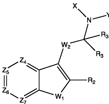
Formula I
