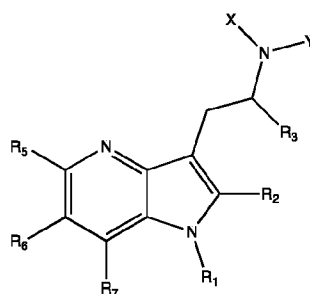
Formula Id
