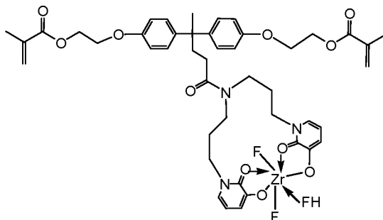
(Compound 18 ) R11L3-ZrF 3 H
