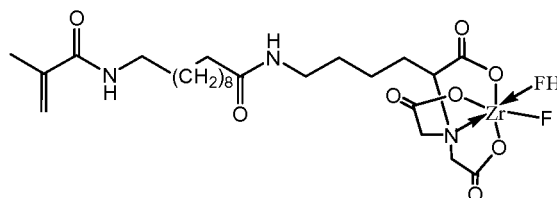
(Compound 4 ) R1L1-ZrF 2 H
