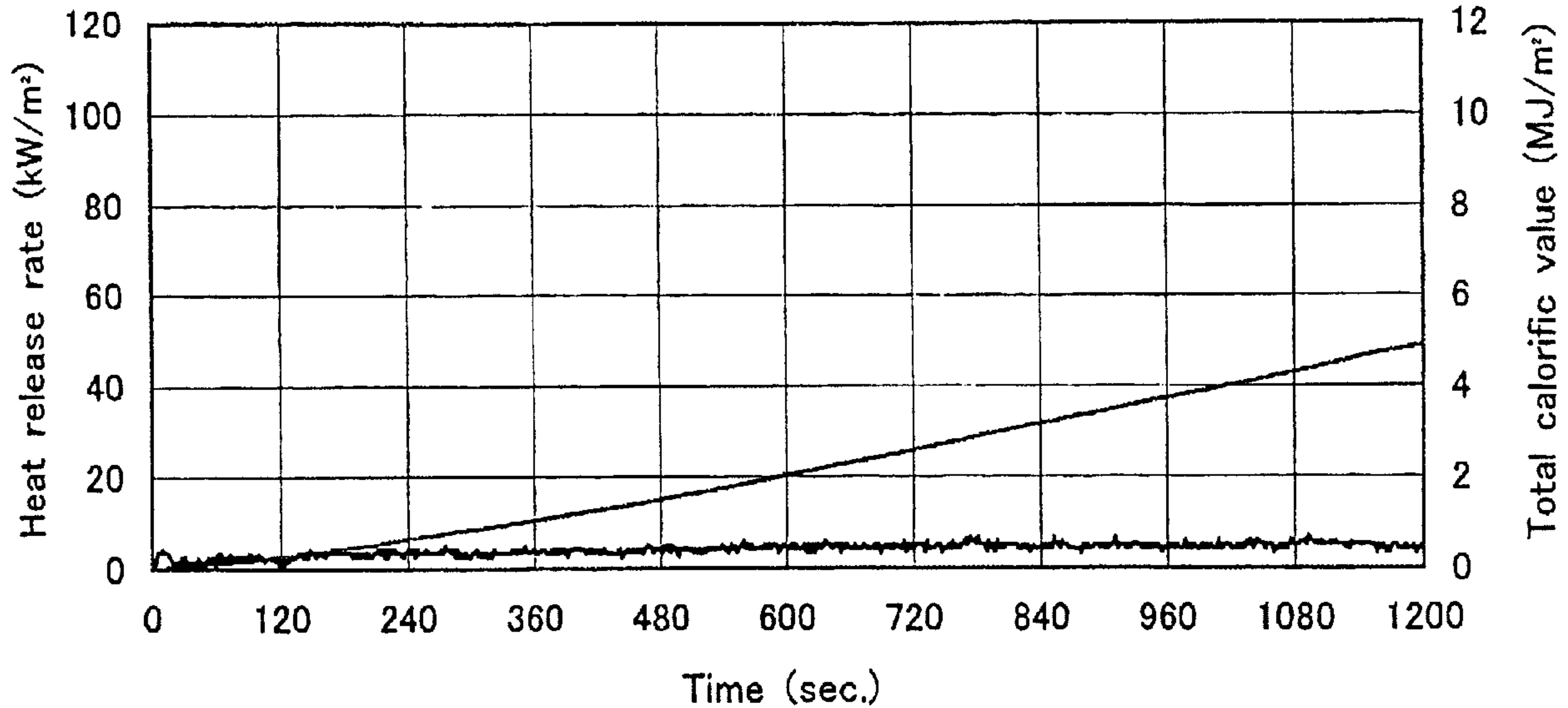
Results of combustion test (Specimen K)
