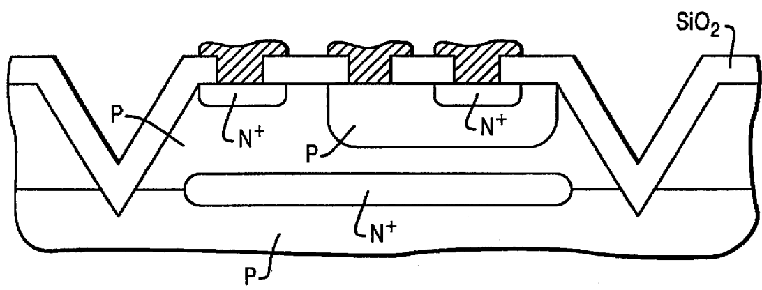
FIG. 4 PRIOR ART
