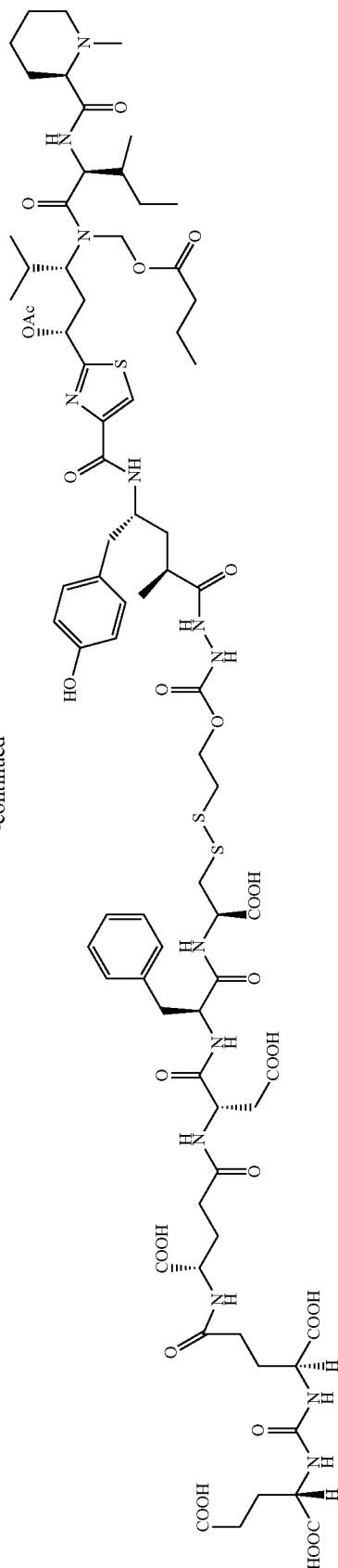
PC01SK71 C_{77}H_{100}N_{13}O_{28}S_3 Mol. Wt.: 1760.35
