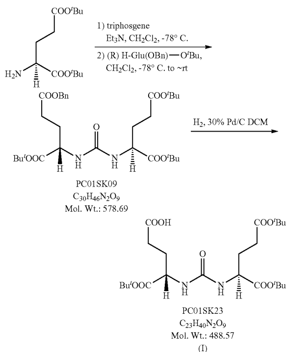
Scheme 2.1
