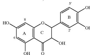
Quercetin
