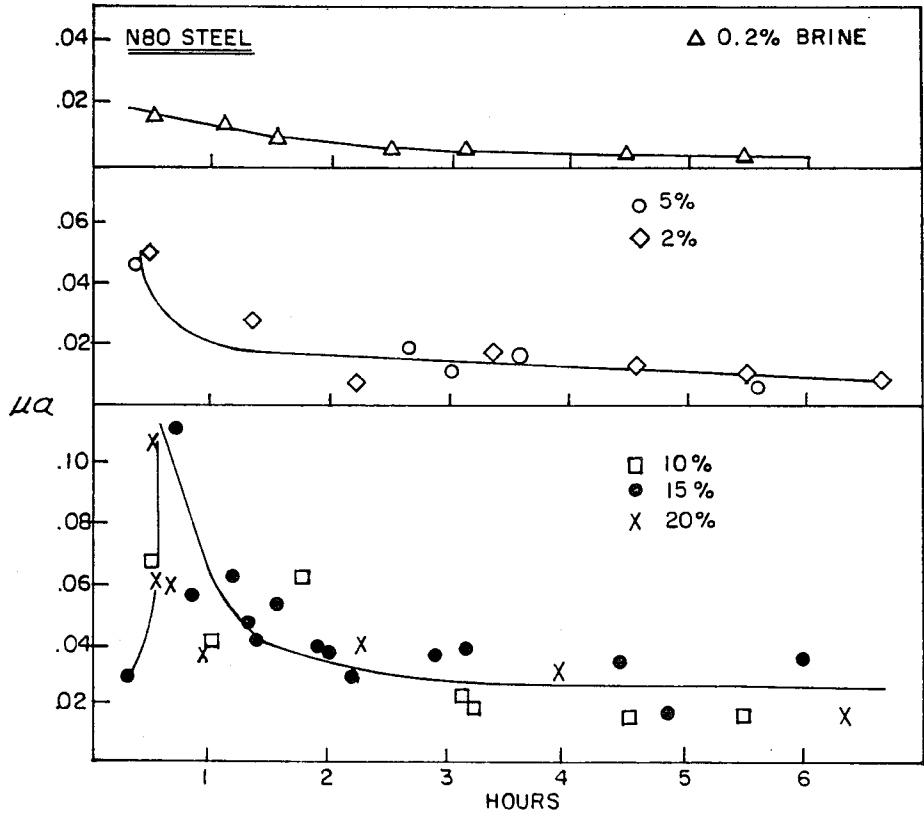
CORROSION CURRENT / TIME PROFILES FOR VARYING % BRINE (4% NaCl ) IN CRUDE C, 760 PSIG CO_2 , 185°F.
