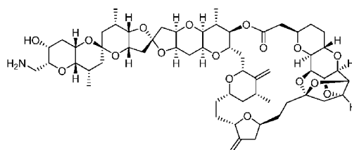
Compound (1)
