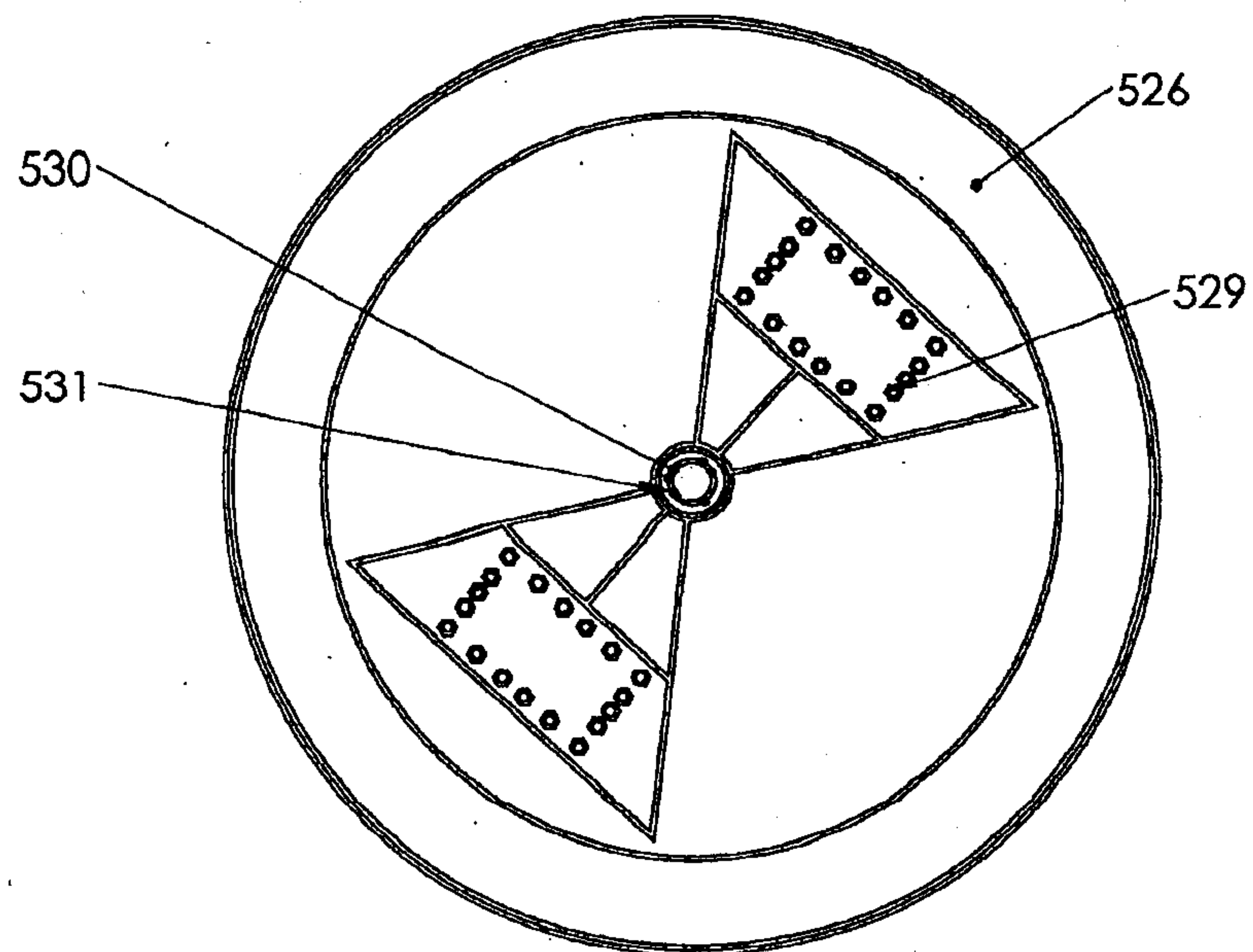
BOTTOM VIEW
