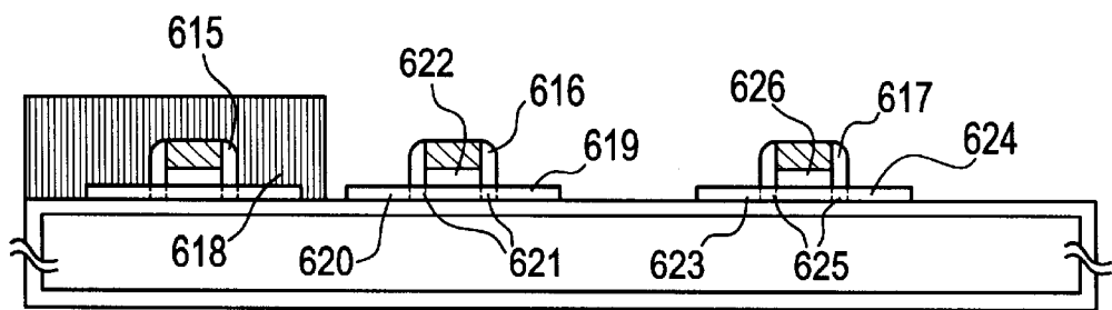
FIG. 7A PHOSPHORUS ADDITION PROCESS
