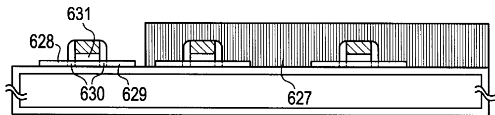
FIG. 7B BORON ADDITION PROCESS
