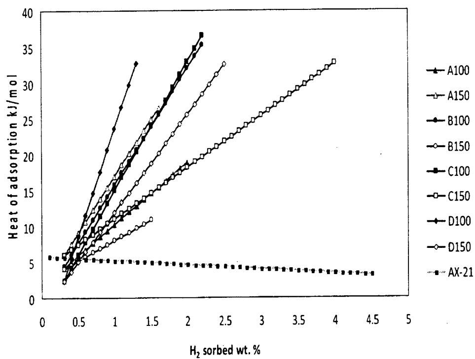
Figure 23: Heat of hydrogen adsorption on vanadium hydrazide materials and carbon AX-21.
