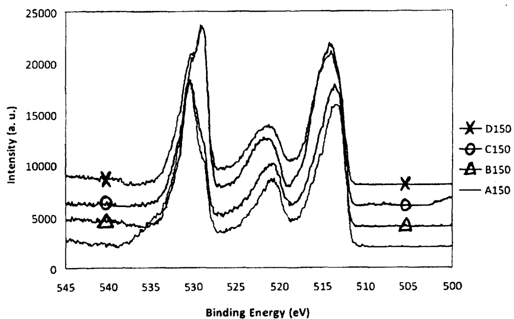
Figure 8: Vanadium 2p 1/2 and 2p 3/2 and oxygen 1s region of XPS spectrum of vanadium hydrazide materials heated to 150 °C with different ratios of hydrazine.
