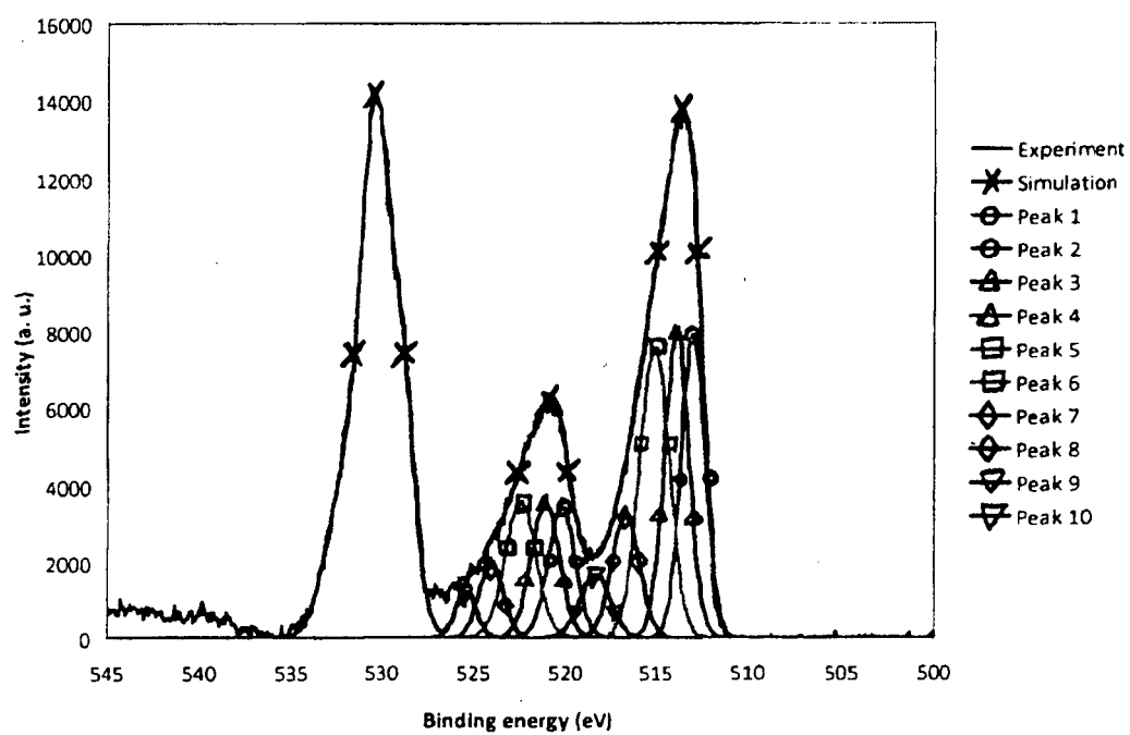
Figure 10: Peak fitting of vanadium 2p 1/2 and 2p 3/2 emissions in the XPS spectrum of B150 sample.
