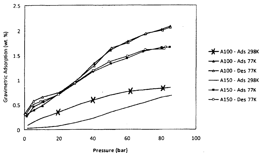
Figure 18: Hydrogen adsorption – desorption excess storage isotherms of A-series vanadium hydrazide materials synthesized with a V:hydrazine ratio of 4:3. Desorption isotherms recorded at 298 K omitted for clarity.
