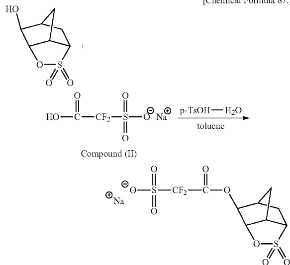
Compound (6)
