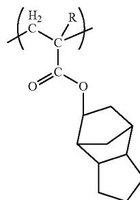
[Chemical Formula 31]
