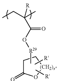
[Chemical Formula 24.]
