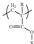
[Chemical Formula 9.]
