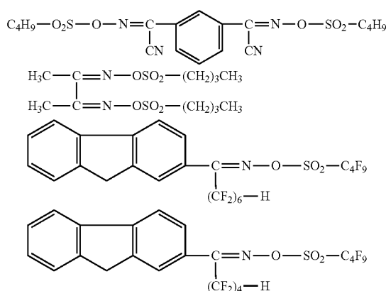
[Chemical Formula 52.]
