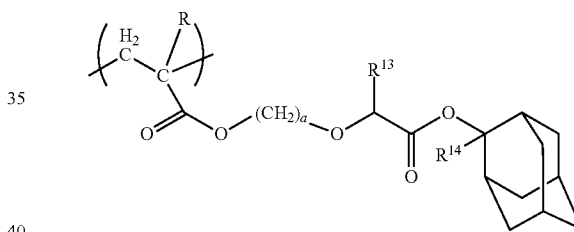
(a1-3-01)
