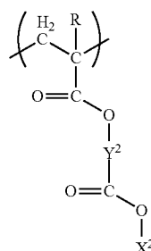
[Chemical Formula 10.]
