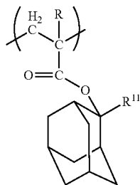
[Chemical Formula 20.]
