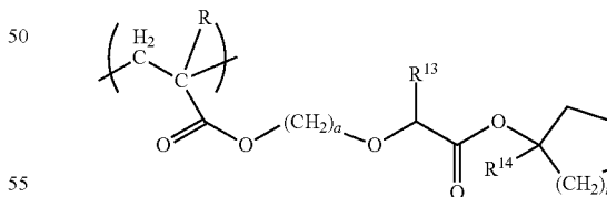
[Chemical Formula 23.]
