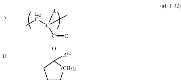
[Chemical Formula 21.]
