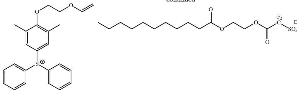
Compound (B1-3)
