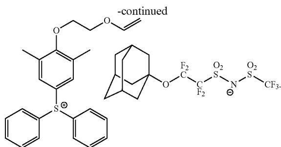
Compound (B1-4')
