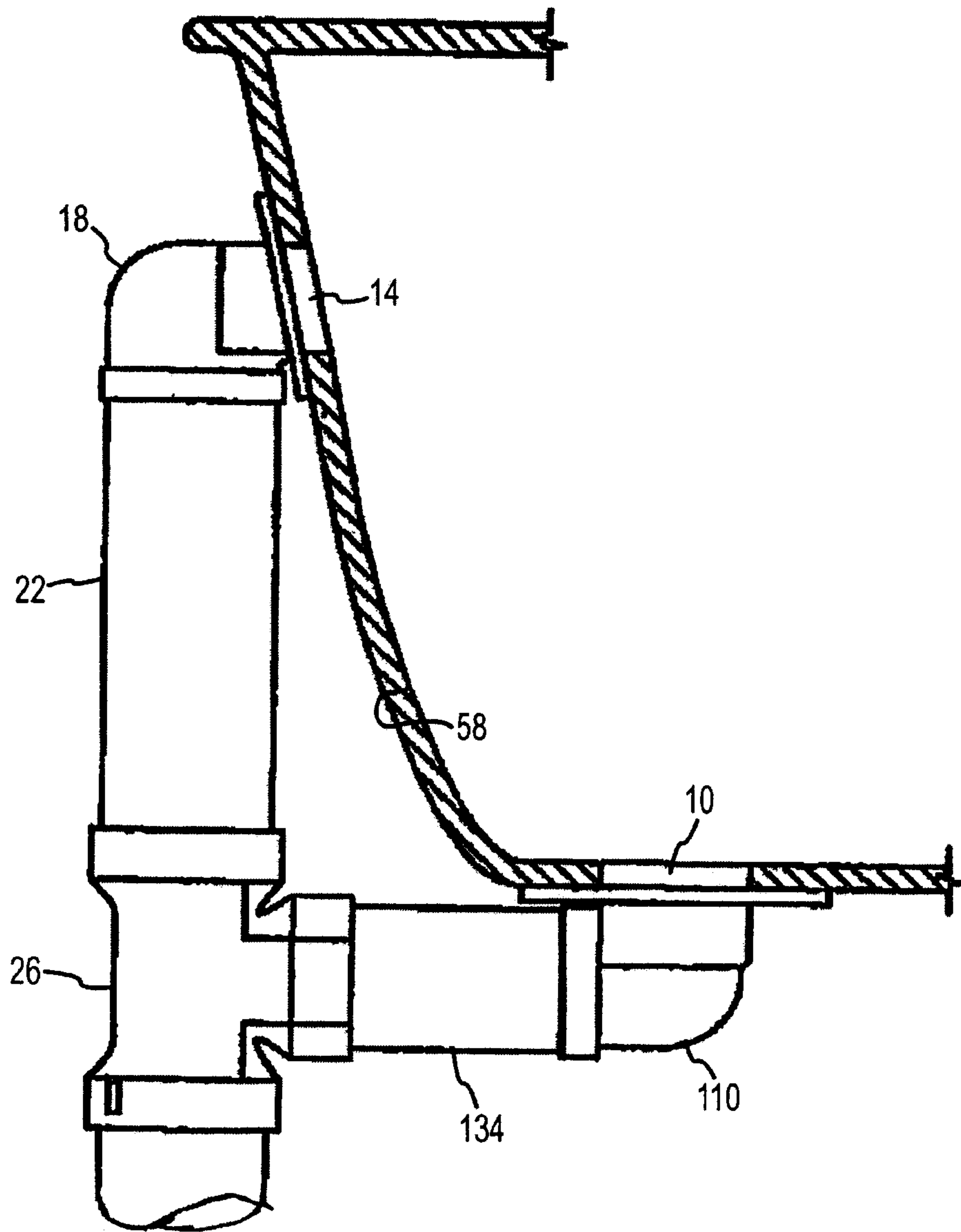
FIG. 12 (PRIOR ART)
