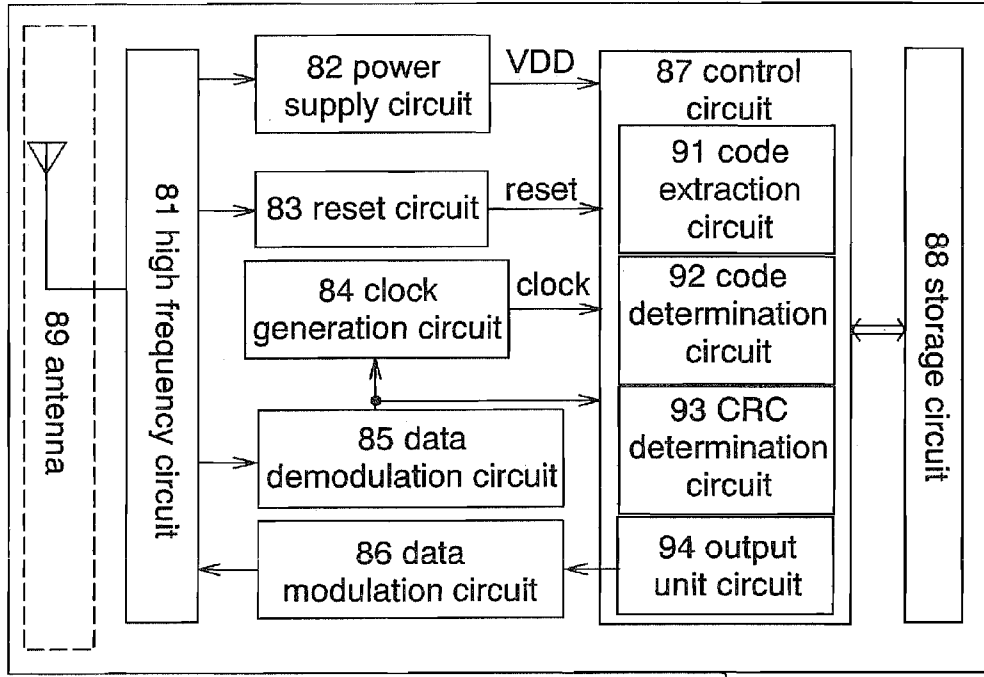
FIG. 13A 80 semiconductor device
