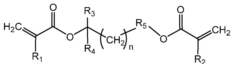
[Chemical Formula 1]
