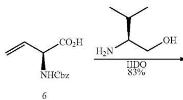
Scheme 2: Synthesis of Syringolin A
