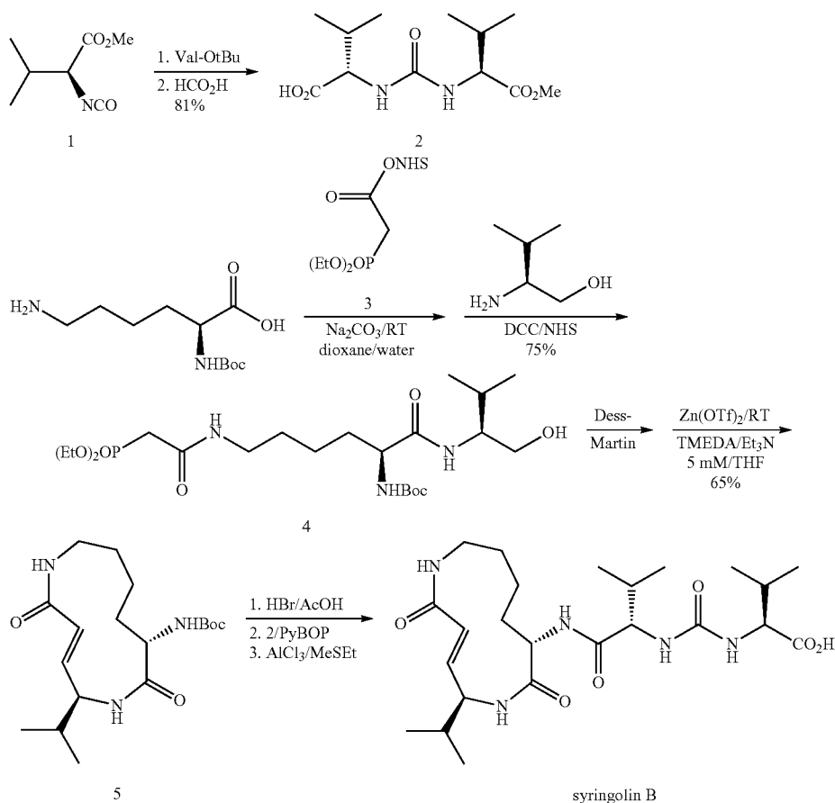
Scheme 1: Synthesis of Syringolin B
