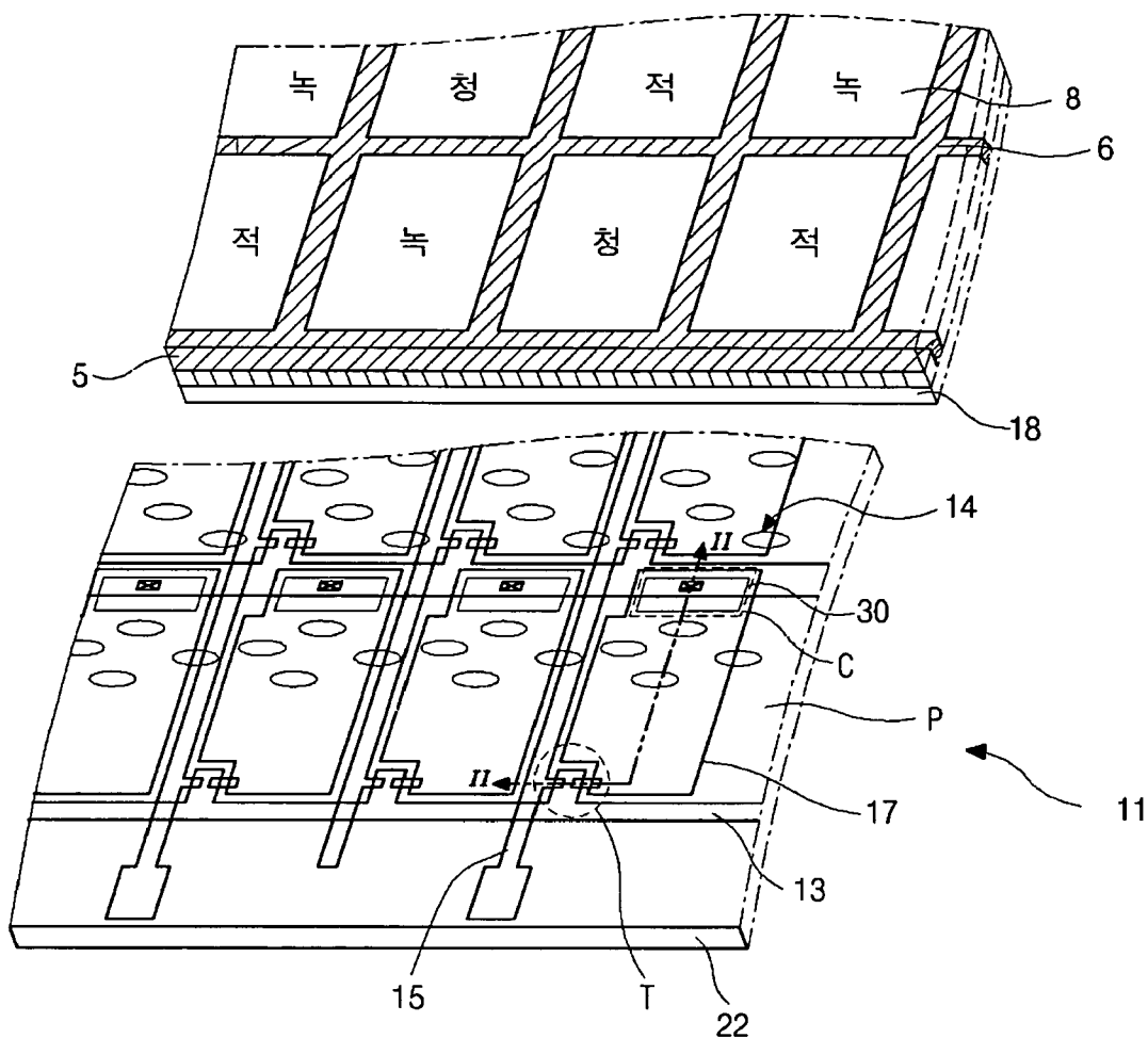
FIG. 1 RELATED ART
