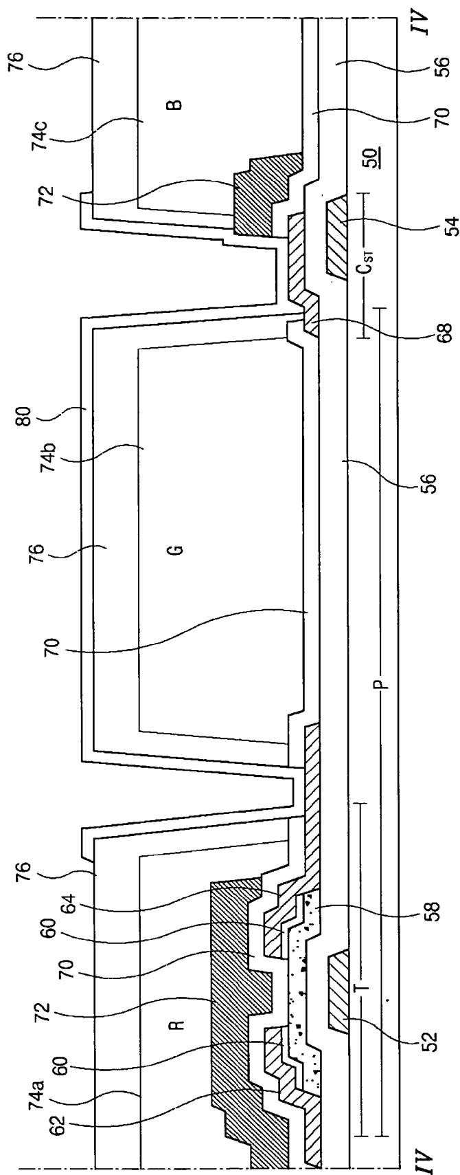
FIG. 3 RELATED ART
