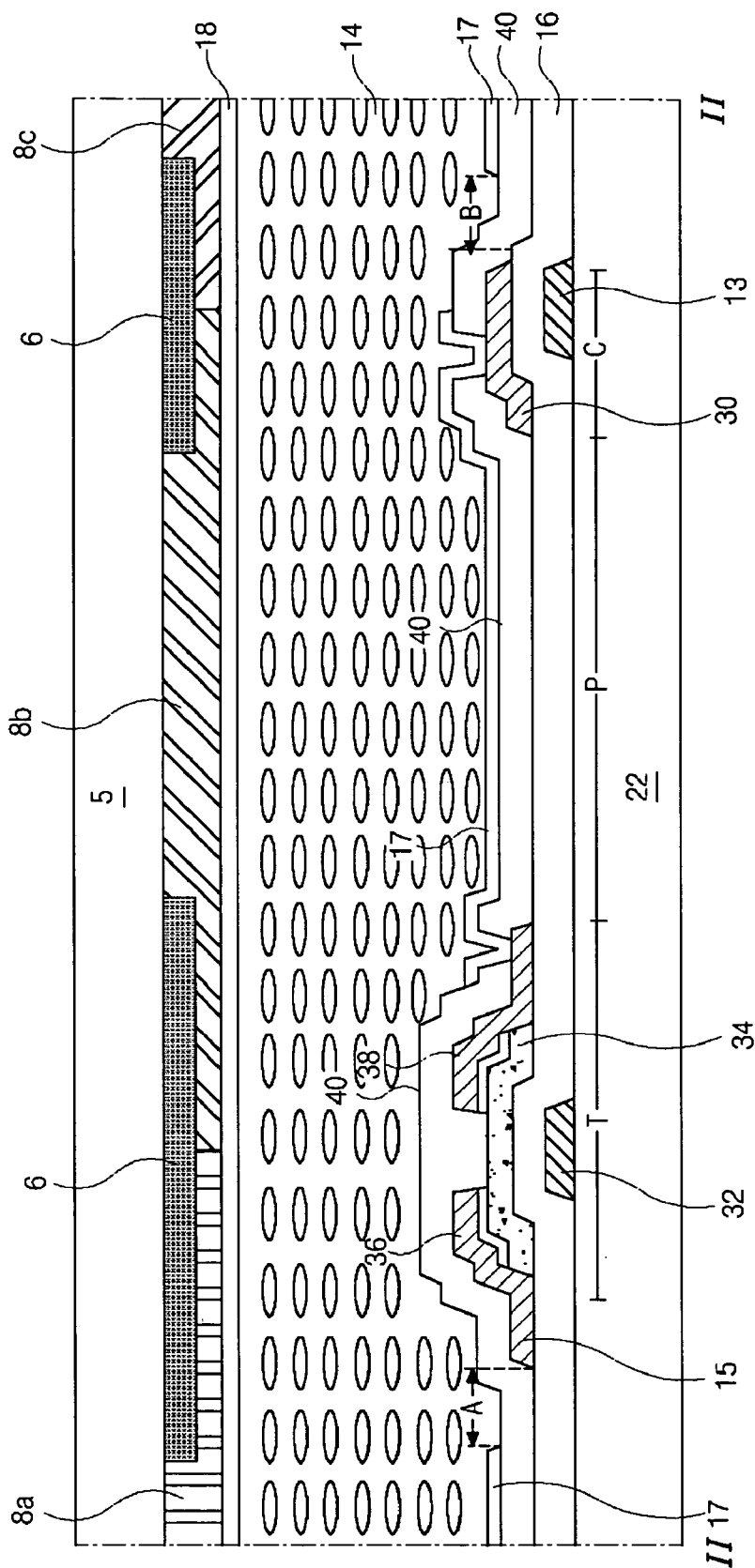
FIG. 2 RELATED ART
