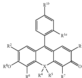
5 [Formula 17]
