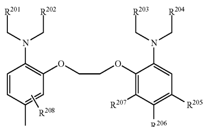
[Formula 16]
