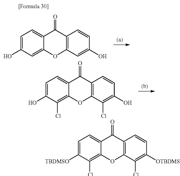
(a) 4,5-Dichloro-3,6-dihydroxyxanthone
