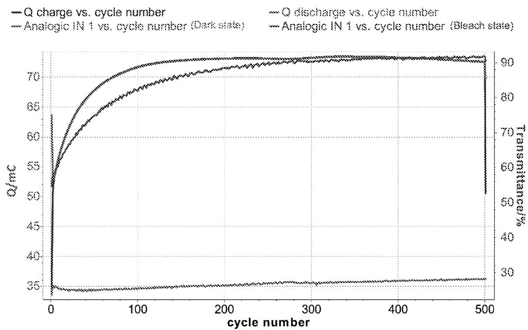
Figure 3 \text{LiNiZrVO}_x ( \sim 200 nm, charge capacity and transmission from CV)
