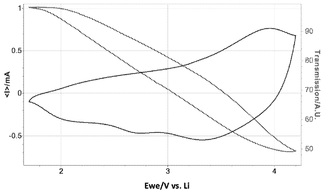
Figure 1 \text{LiNiZrVO}_x (~80 nm, CV, 50 th cycle)
