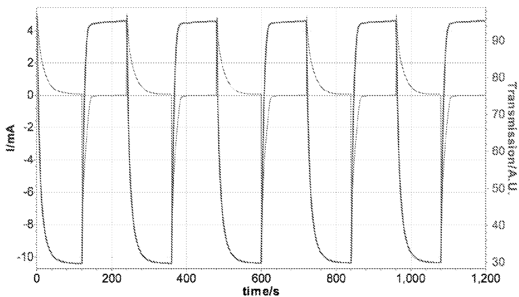
Figure 2 \text{LiNiZrVO}_x (~200 nm, CA, after 500 CV cycles)
