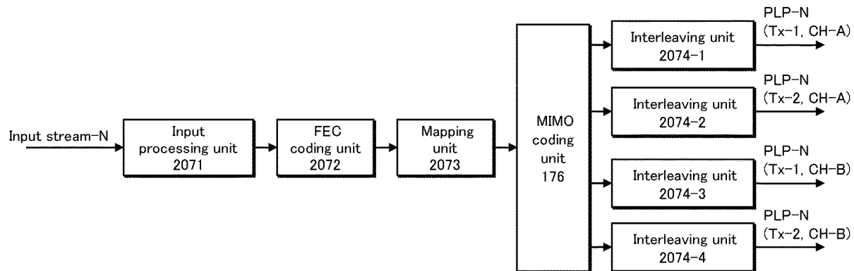
MIMO-PLP processing unit 131-N
