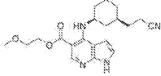
Cis-enantiomer 1
