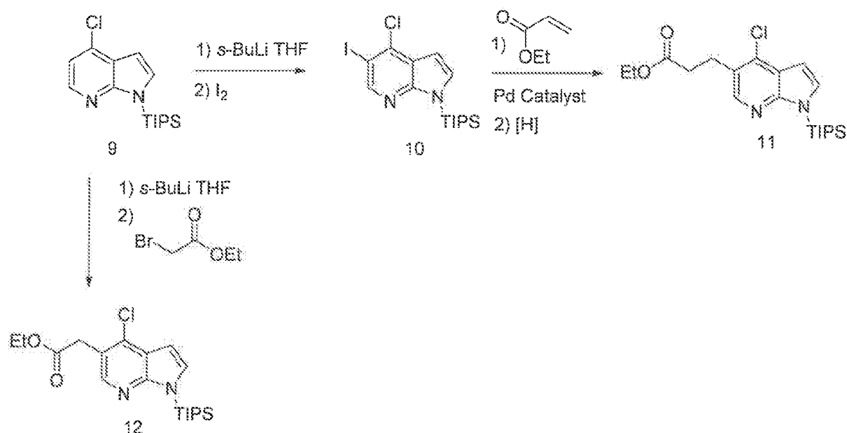
Scheme 3. Preparation of 5-Alkyl-ester Pyrrolopyridines.
