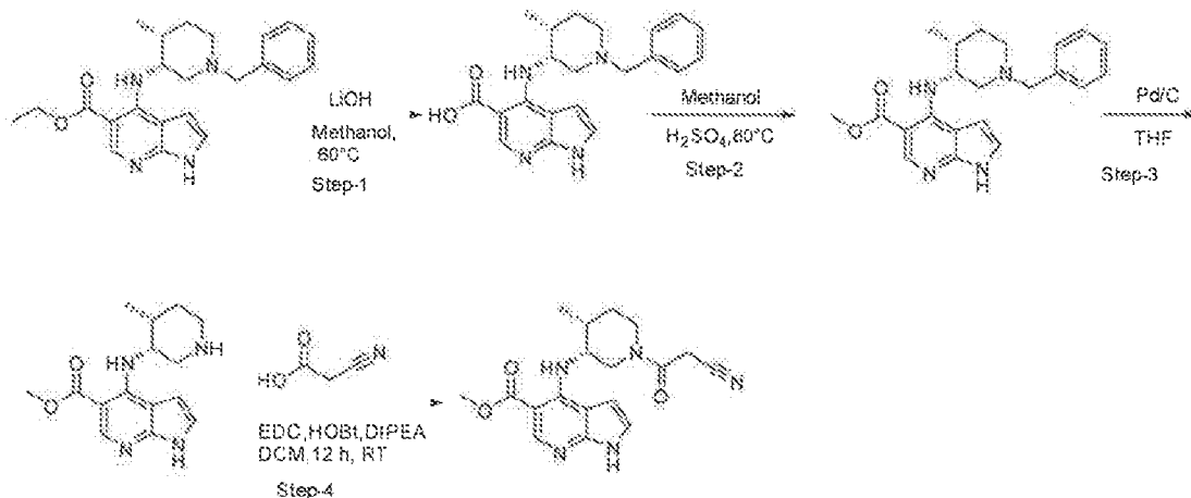
Scheme 18. Preparation of methyl 4-(((3 R ,4 R )-1-(2-cyanoacetyl)-4-methylpiperidin-3-yl)amino)-1 H -pyrrolo[2,3- b ]pyridine-5-carboxylate.
