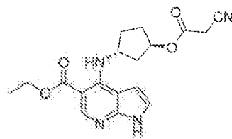
Trans, enantiomer-2
