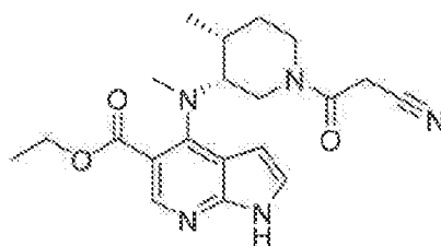
Scheme 6. Preparation of ethyl 4-(((3 R ,4 R )-1-(2-cyanoacetyl)-4-methylpiperidin-3-yl)(methylamino)-1 H -pyrrolo[2,3- b ]pyridine-5-carboxylate
