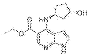
Trans, Racemic
