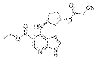
Trans, Racemic
