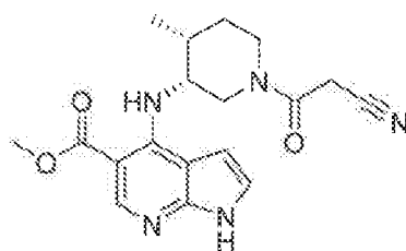
Scheme 18. Preparation of methyl 4-(((3 R ,4 R )-1-(2-cyanoacetyl)-4-methylpiperidin-3-yl)amino)-1 H -pyrrolo[2,3- b ]pyridine-5-carboxylate.
