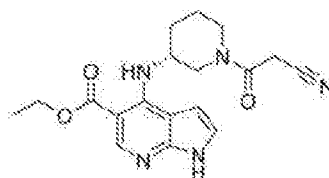
Scheme 17. Preparation of ethyl ( R )-4-((1-(2-cyanoacetyl)piperidin-3-yl)amino)-1 H -pyrrolo[2,3- -150-
