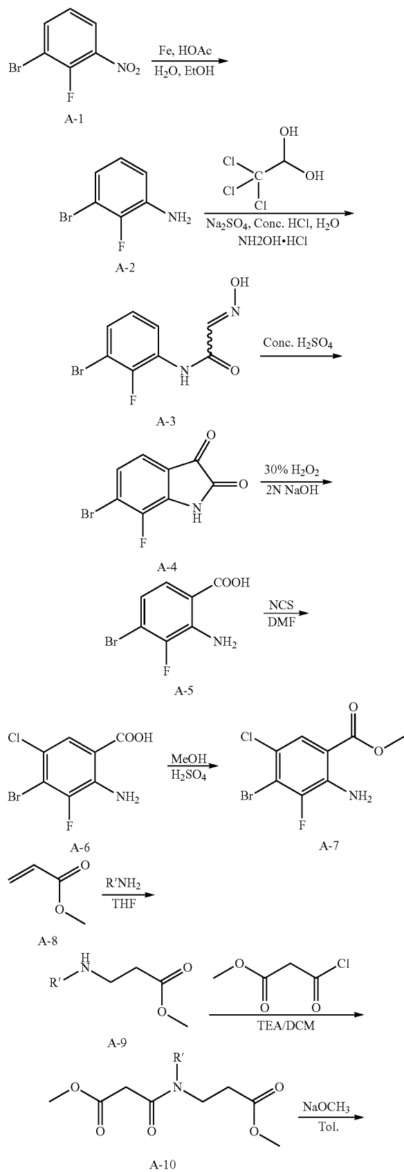
General Reaction Scheme 1
