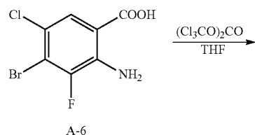
General Reaction Scheme 2
