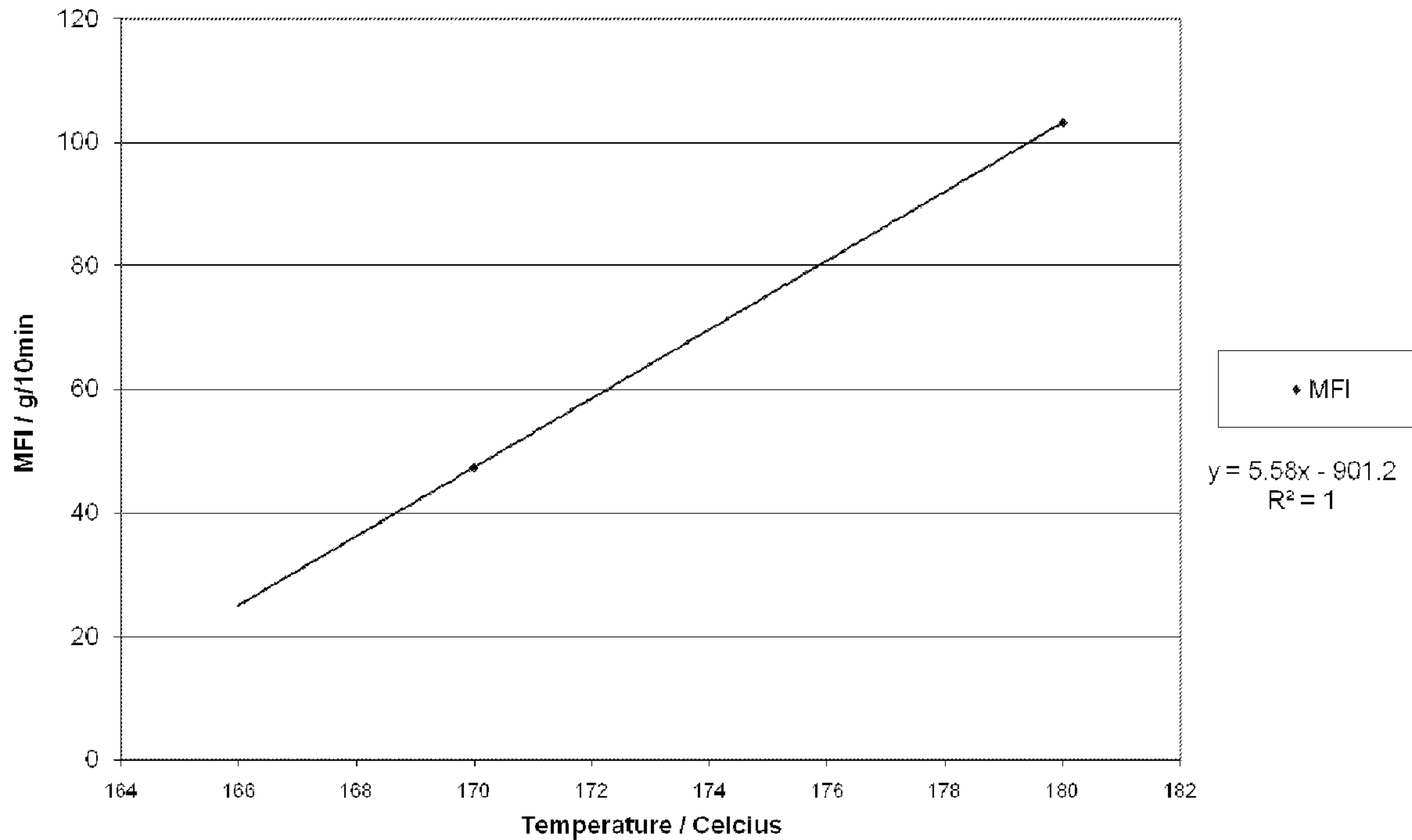
45% DDS, 55% KM180, MFI vs Temperature
