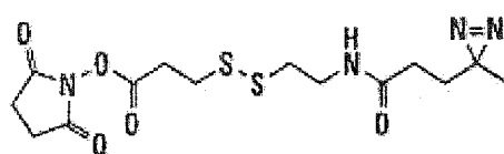
SDAD (NHS-SS-Diazirine) M.W. 388.46 Spacer Arm 13.5 Å
