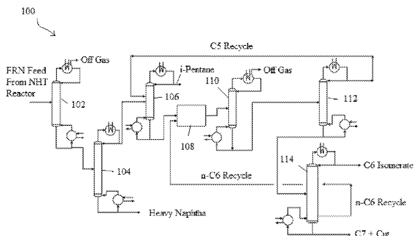
FIGURE 1 (Prior Art)
