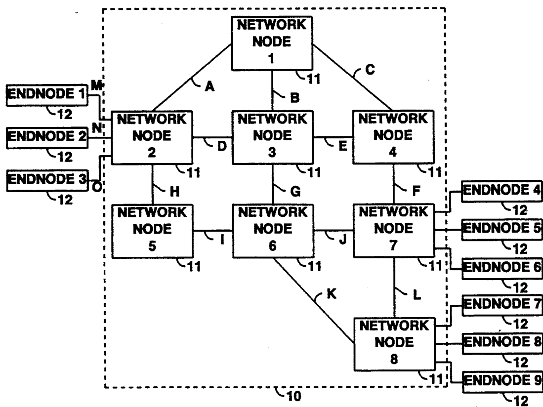
PACKET COMMUNICATIONS NETWORK
