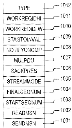
TRANSMIT FIFO ENTRY FORMAT 1000
